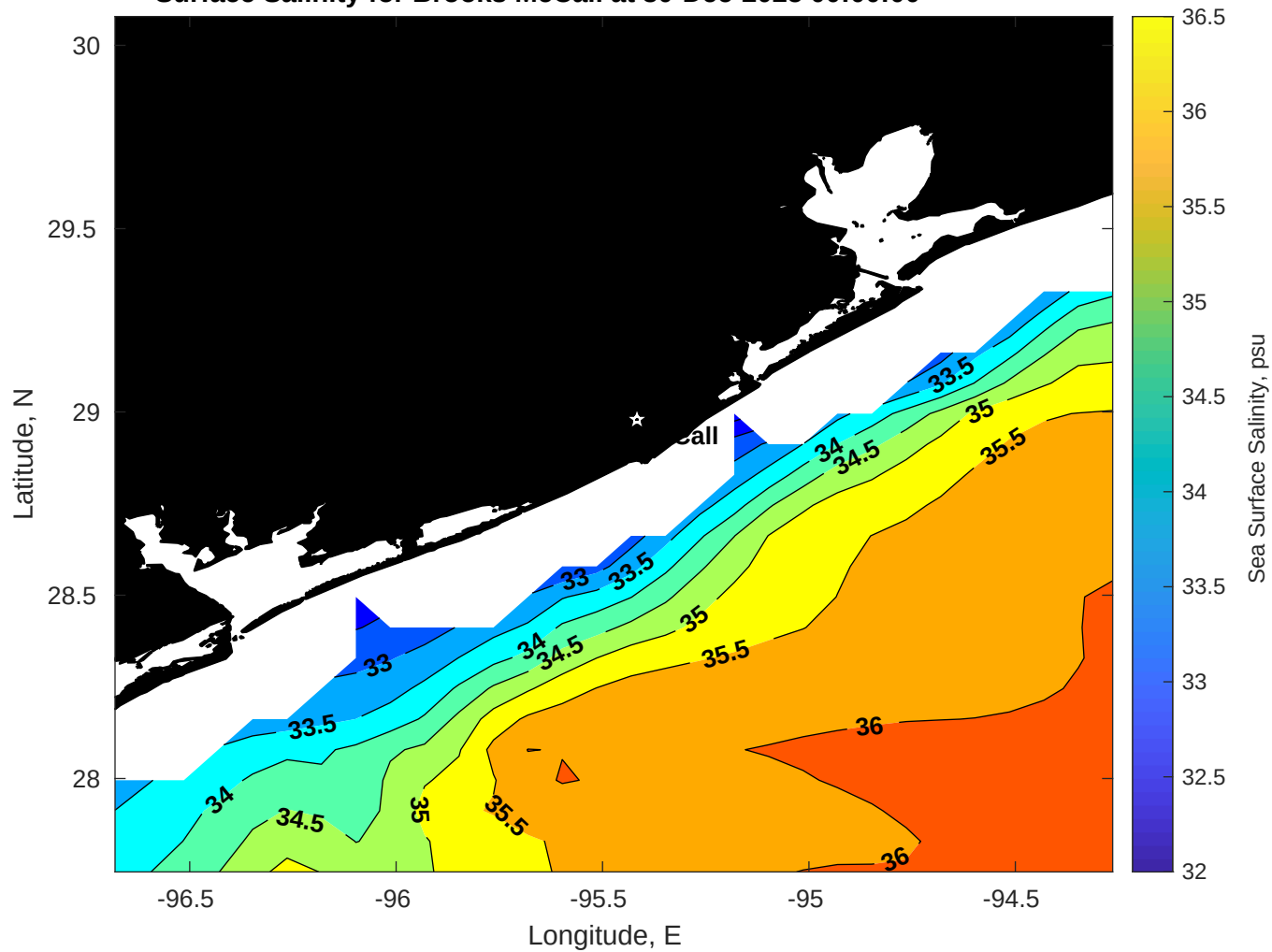
Surface Salinity for Brooks McCall at 30-Dec-2025 00:00:00
