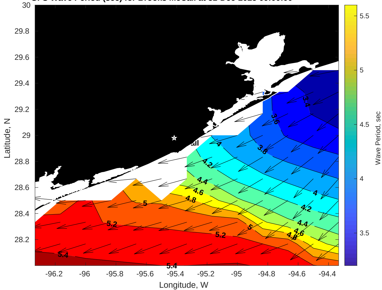
GFS Wave Period (sec) for Brooks McCall at 31-Dec-2025 09:00:00
