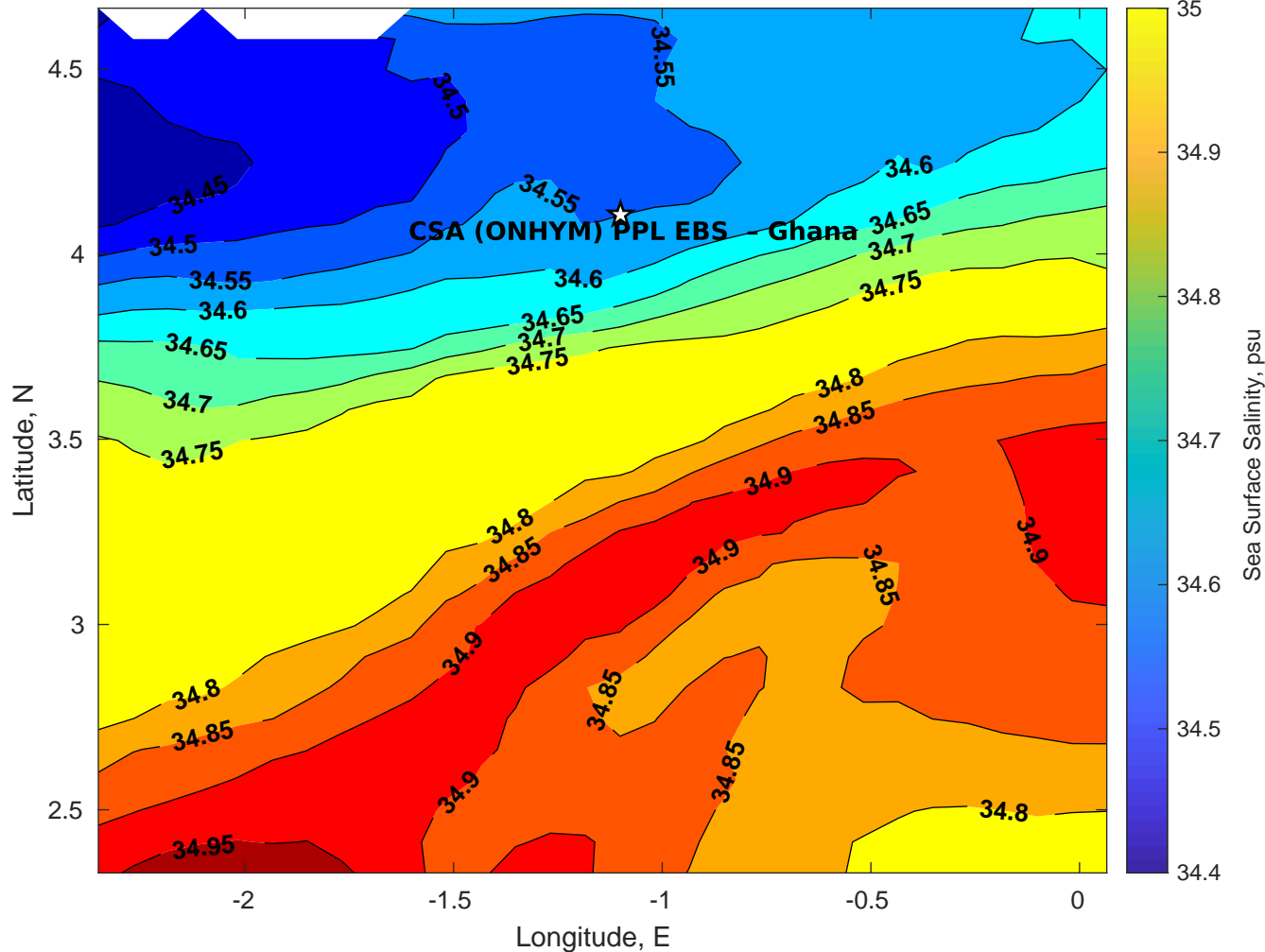
Surface Salinity for CSA (ONHYM) PPL EBS - Ghana at 30-Dec-2025 00:00:00
