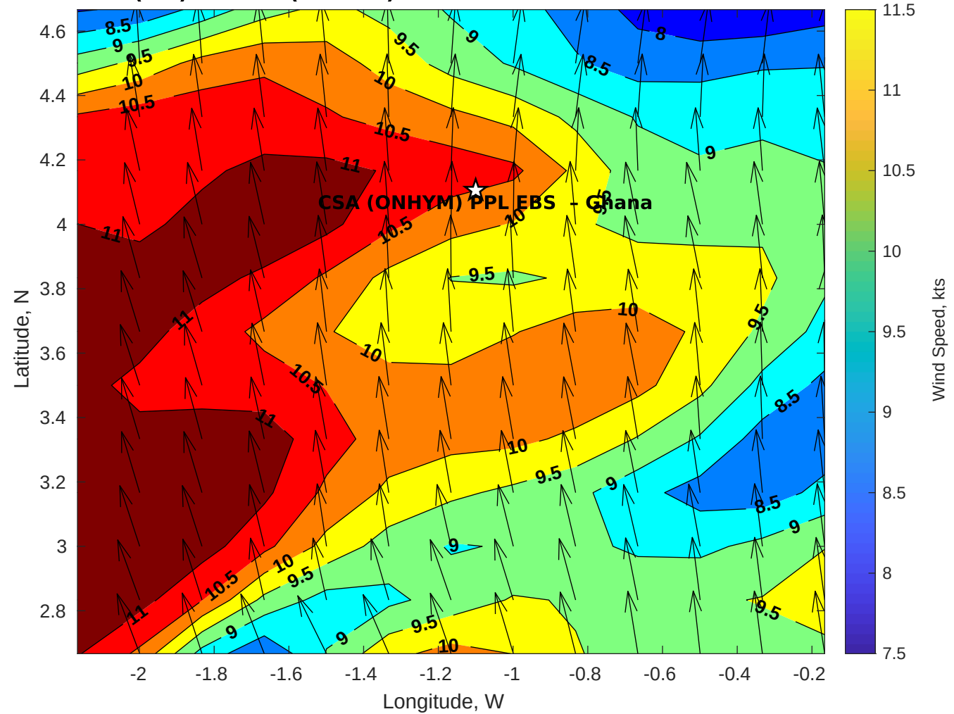
GFS Winds (kts) for CSA (ONHYM) PPL EBS - Ghana at 31-Dec-2025 09:00:00
