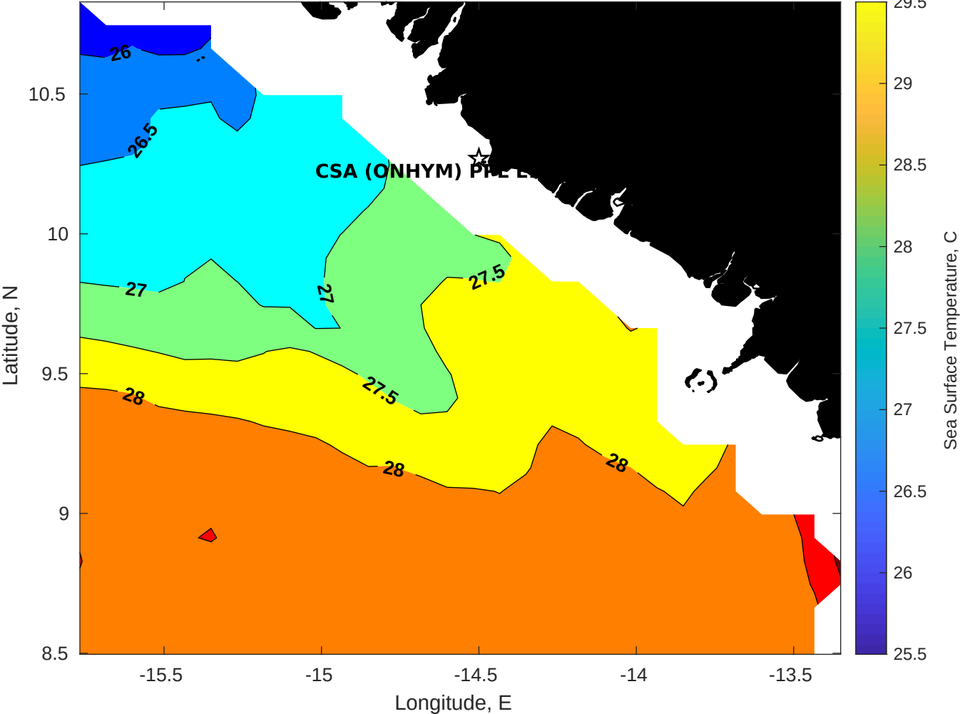
SST for CSA (ONHYM) PPL EBS - Guinea at 30-Dec-2025 00:00:00
