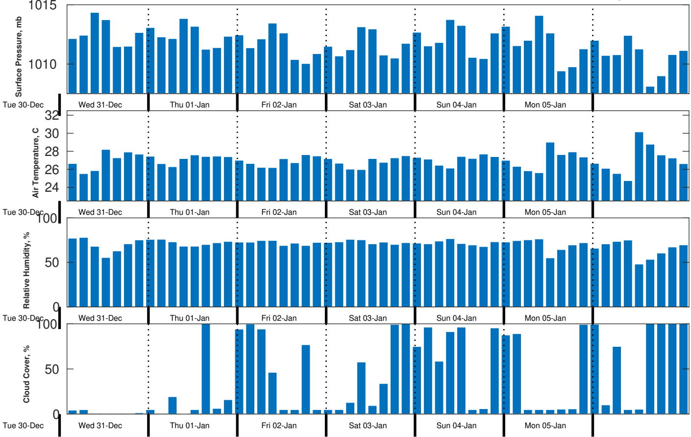
Met Forecast for CSA (ONHYM) PPL EBS - Guinea from 31-Dec-2025 00:00:00 to 07-Jan-2026 00:00:00
