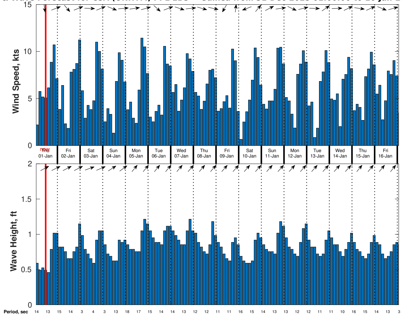
Wind & Wave Forecast for CSA (ONHYM) PPL EBS - Guinea from 31-Dec-2025 01:00:00 to 16-Jan-2026 01:00:00
