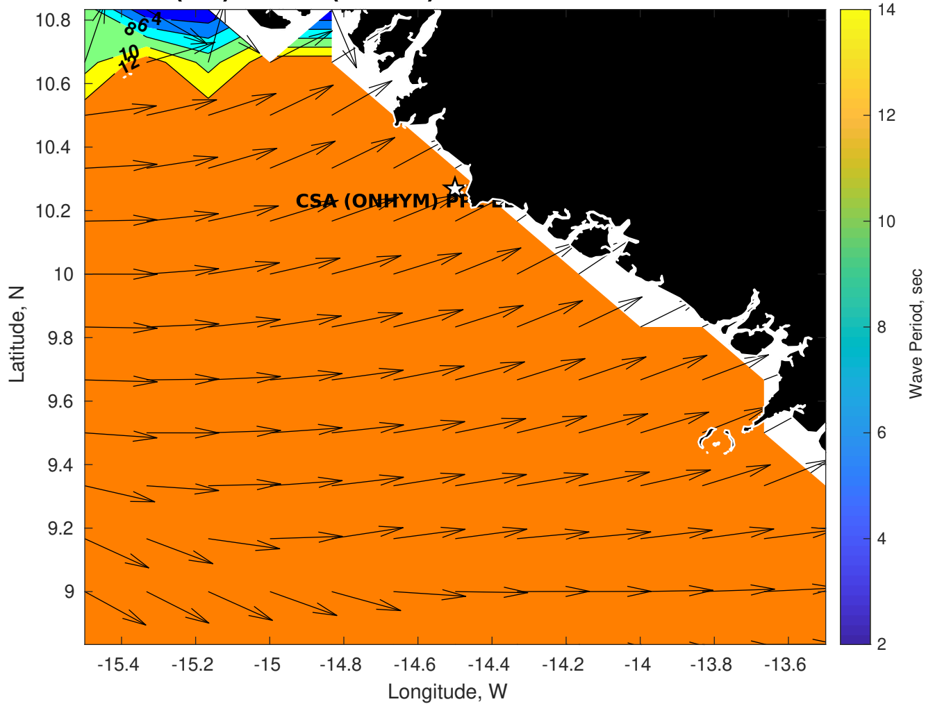
GFS Wave Period (sec) for CSA (ONHYM) PPL EBS - Guinea at 31-Dec-2025 09:00:00
