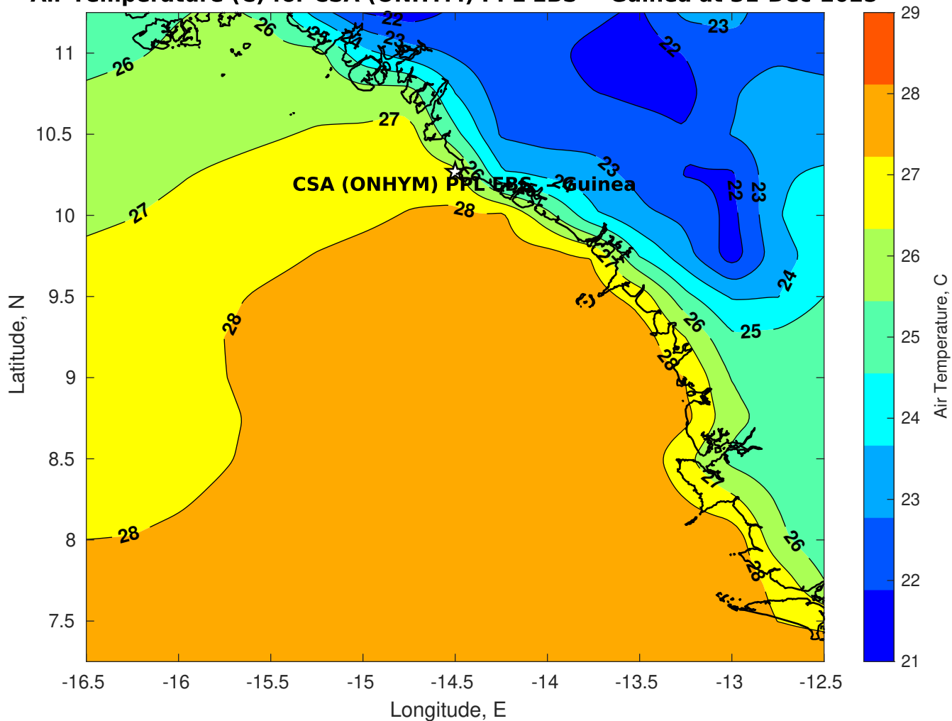
Air Temperature (C) for CSA (ONHYM) PPL EBS - Guinea at 31-Dec-2025
