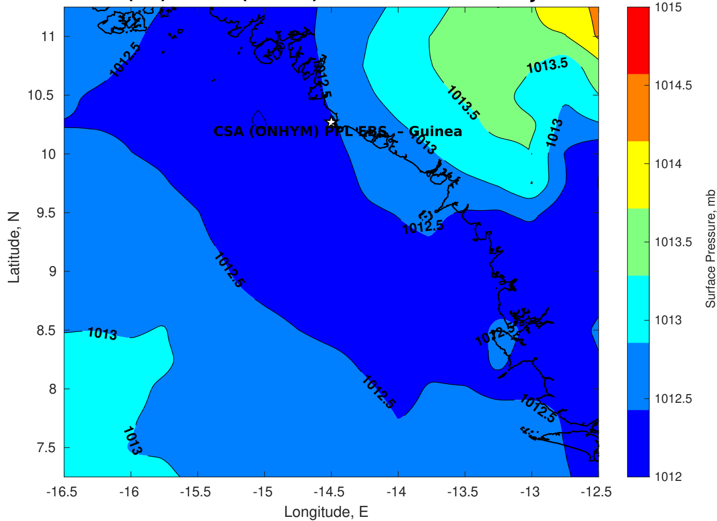
Surface Pressure (mb) for CSA (ONHYM) PPL EBS - Guinea at 02-Jan-2026 00:00:00
