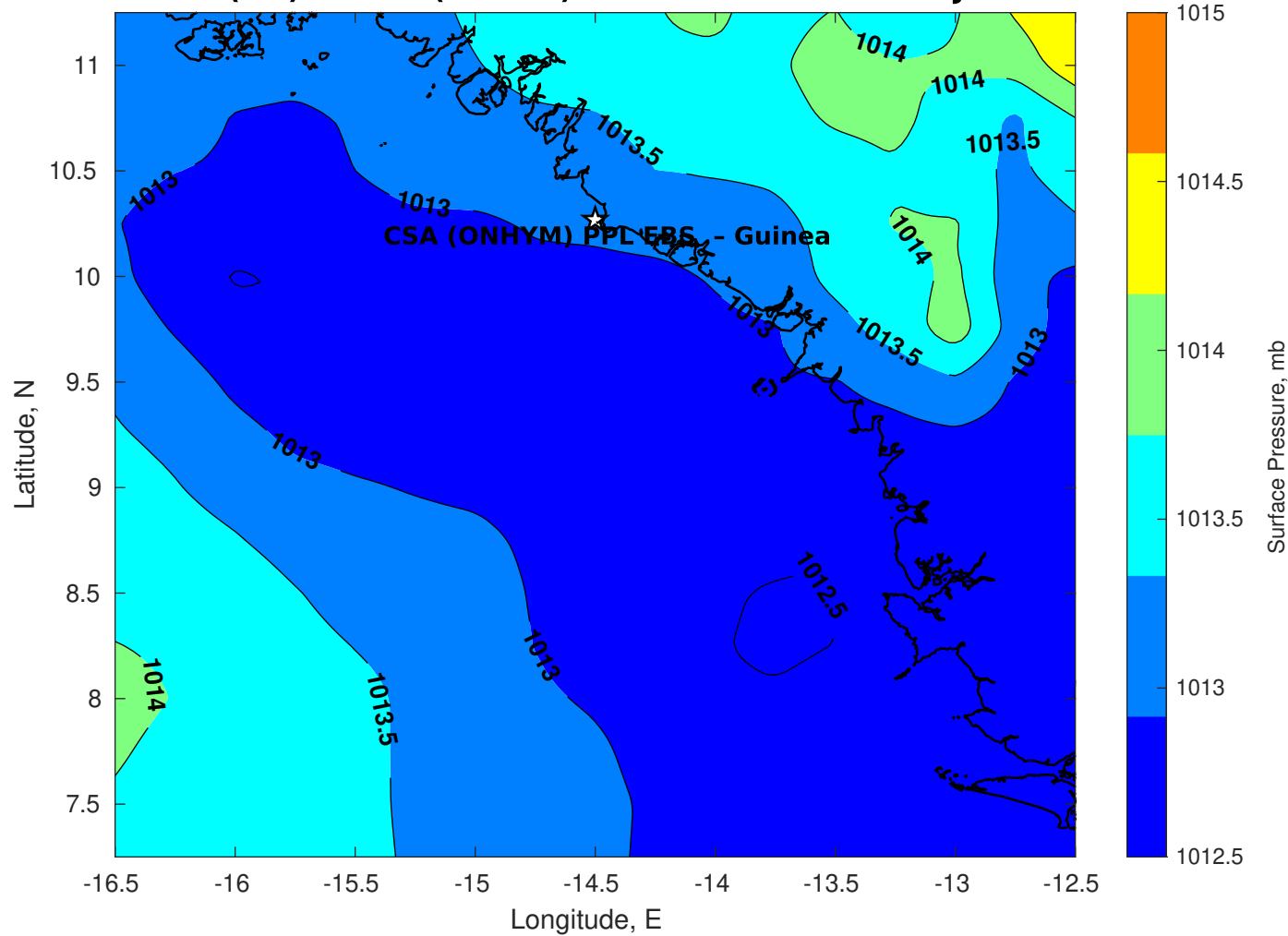
Surface Pressure (mb) for CSA (ONHYM) PPL EBS - Guinea at 01-Jan-2026 00:00:00
