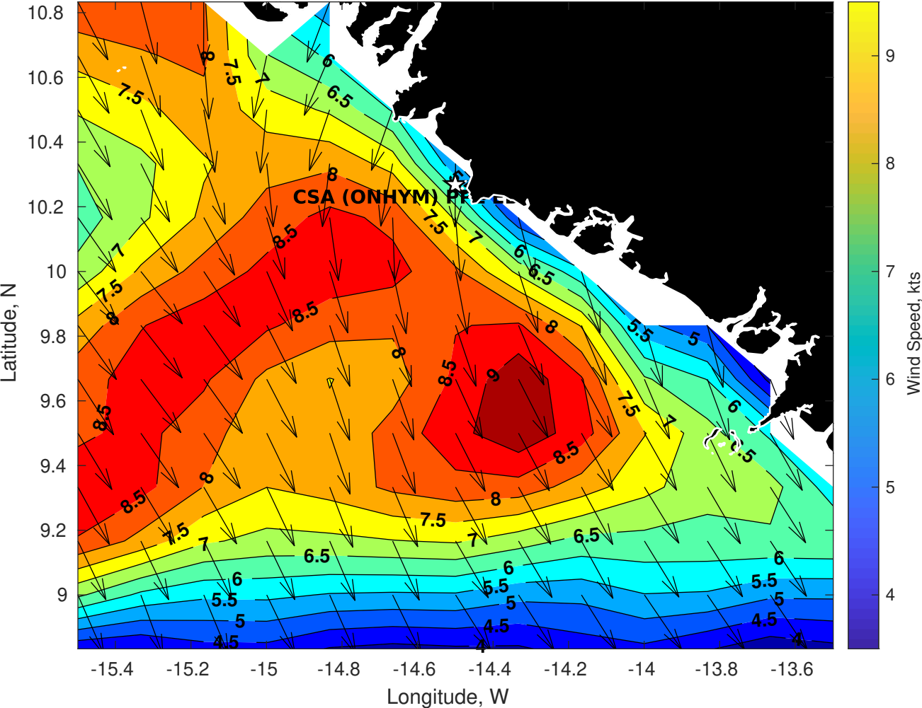
GFS Winds (kts) for CSA (ONHYM) PPL EBS - Guinea at 31-Dec-2025 09:00:00
