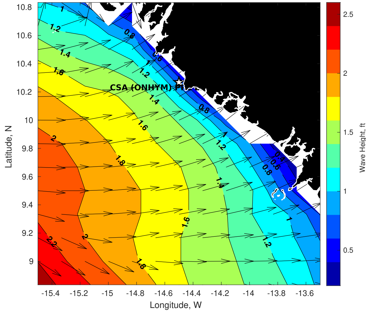
GFS Wave Height (ft) for CSA (ONHYM) PPL EBS - Guinea at 31-Dec-2025 09:00:00
