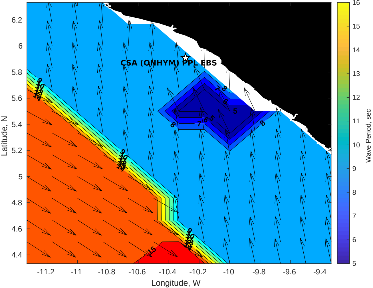
GFS Wave Period (sec) for CSA (ONHYM) PPL EBS - Liberia at 31-Dec-2025 09:00:00
