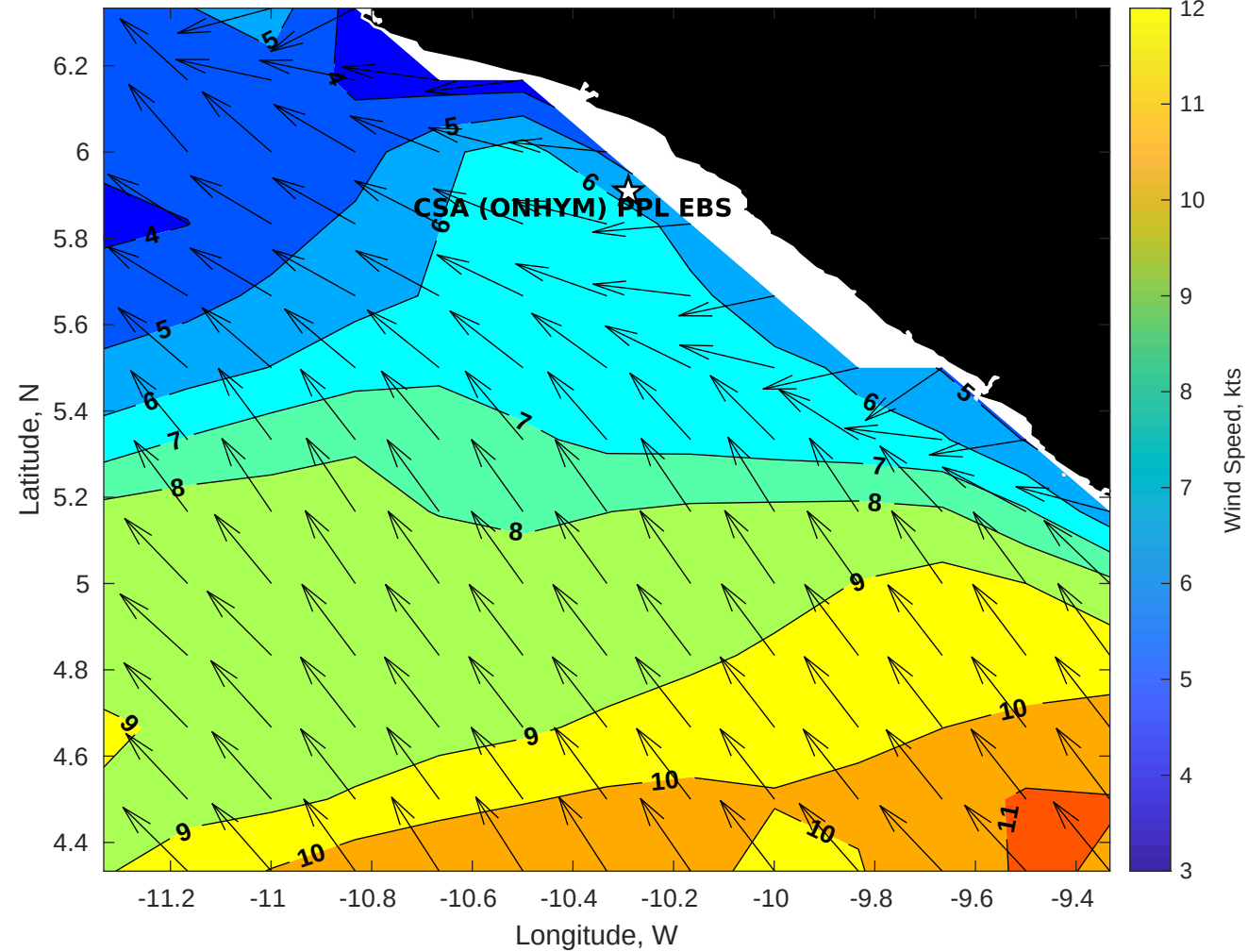
GFS Winds (kts) for CSA (ONHYM) PPL EBS - Liberia at 31-Dec-2025 09:00:00
