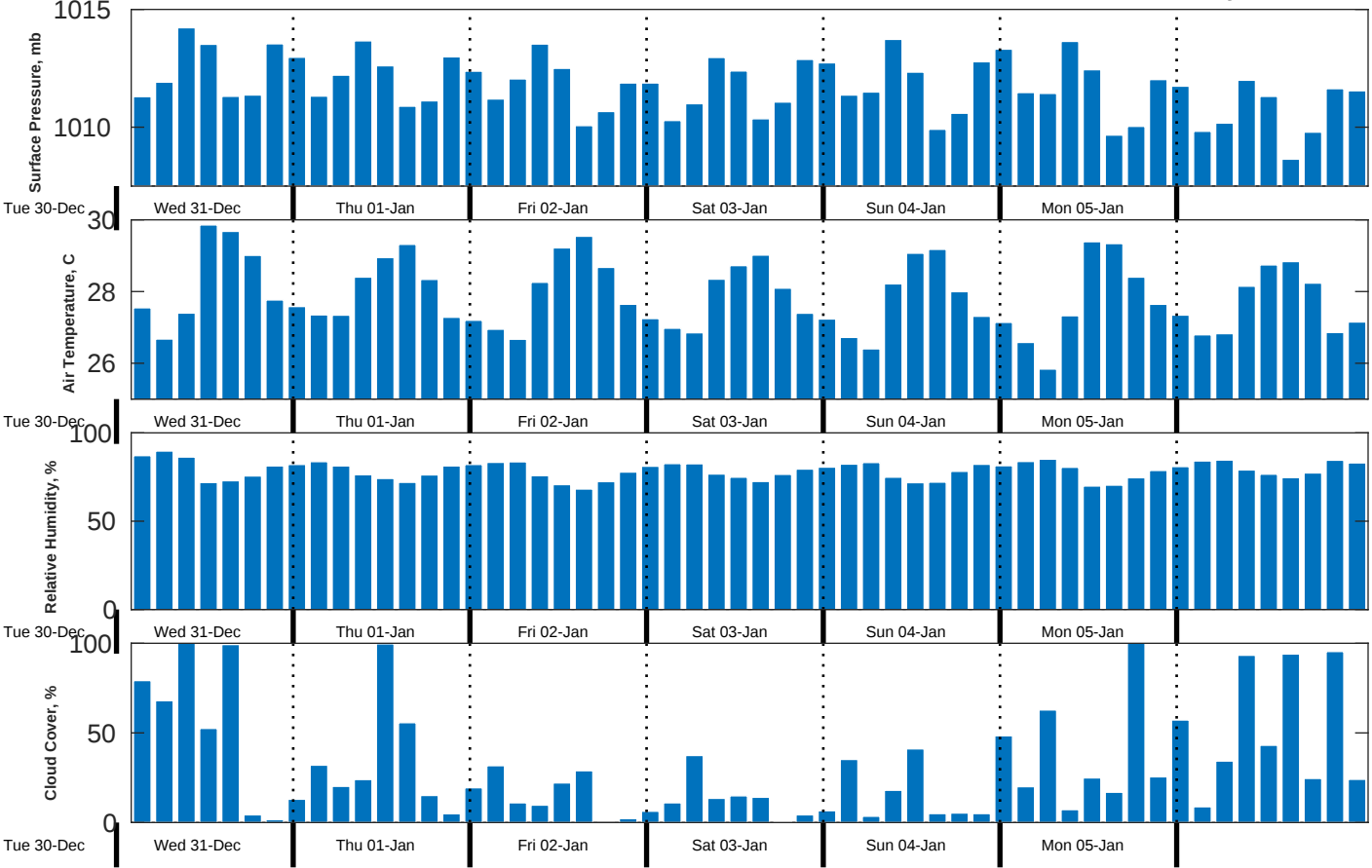
Met Forecast for CSA (ONHYM) PPL EBS - Liberia from 31-Dec-2025 00:00:00 to 07-Jan-2026 00:00:00
