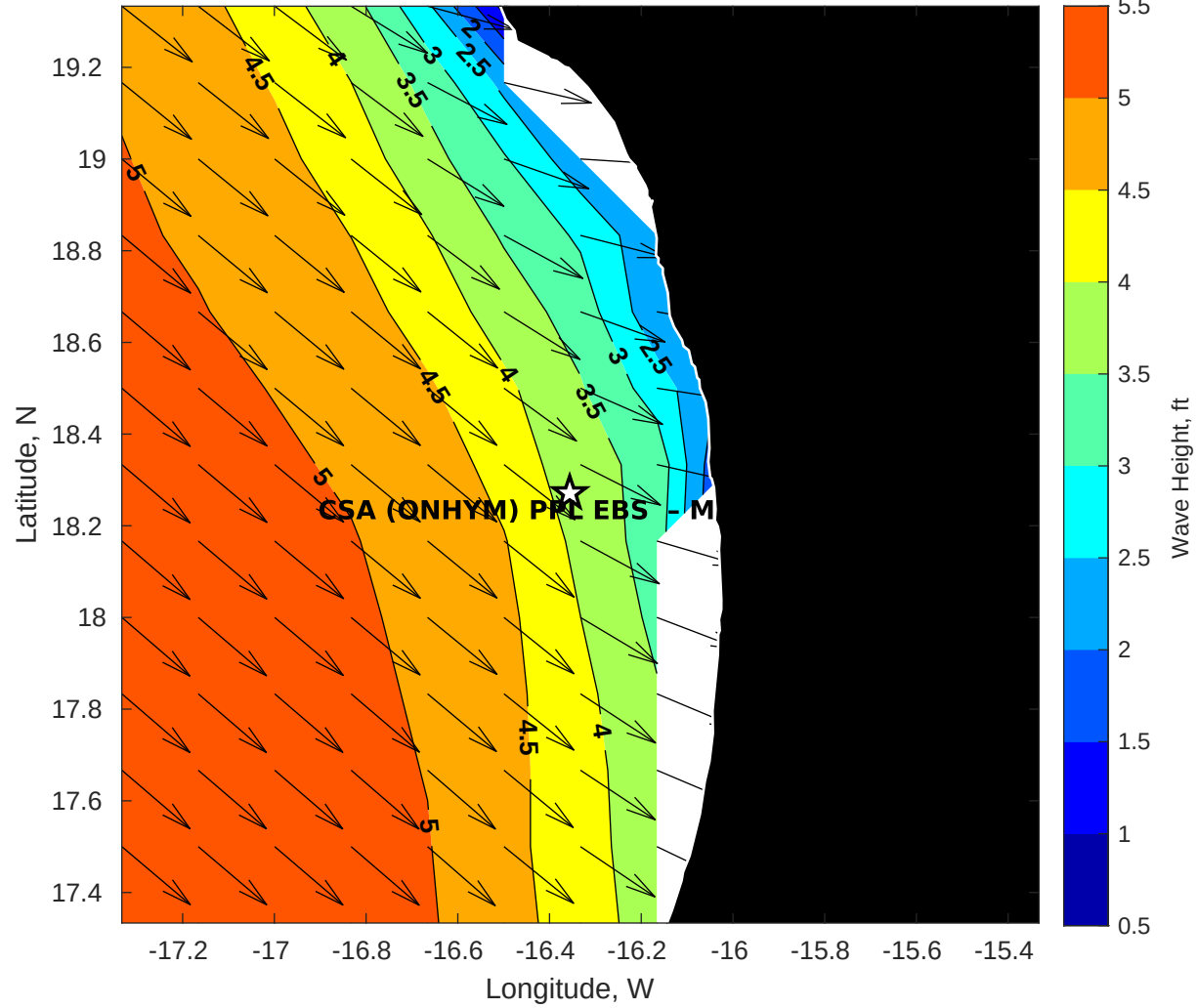
GFS Wave Height (ft) for CSA (ONHYM) PPL EBS - Mauritania at 31-Dec-2025 09:00:00
