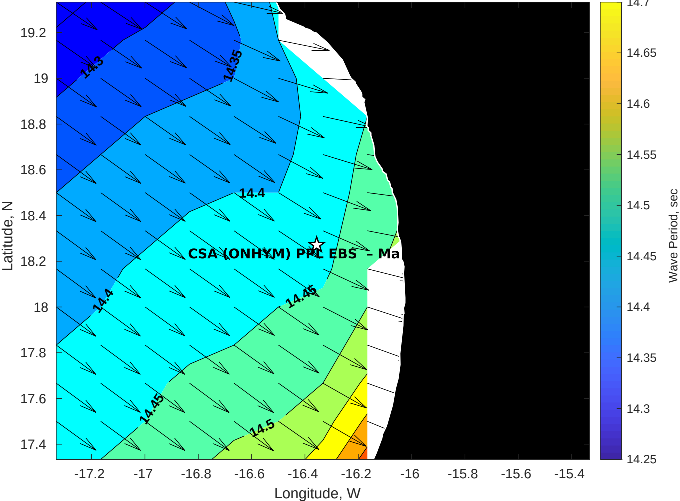
GFS Wave Period (sec) for CSA (ONHYM) PPL EBS - Mauritania at 31-Dec-2025 09:00:00
