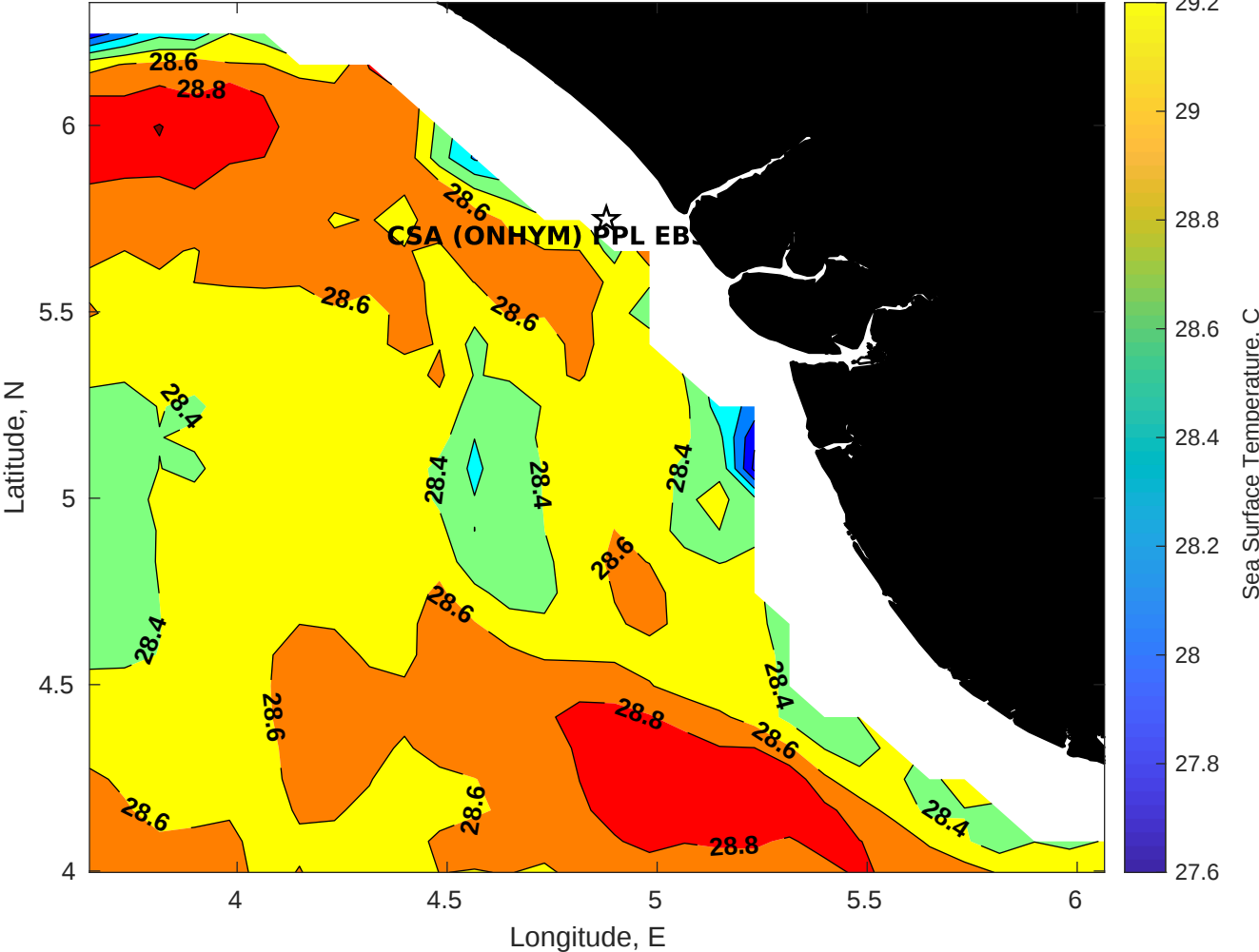
SST for CSA (ONHYM) PPL EBS - Nigeria at 30-Dec-2025 00:00:00
