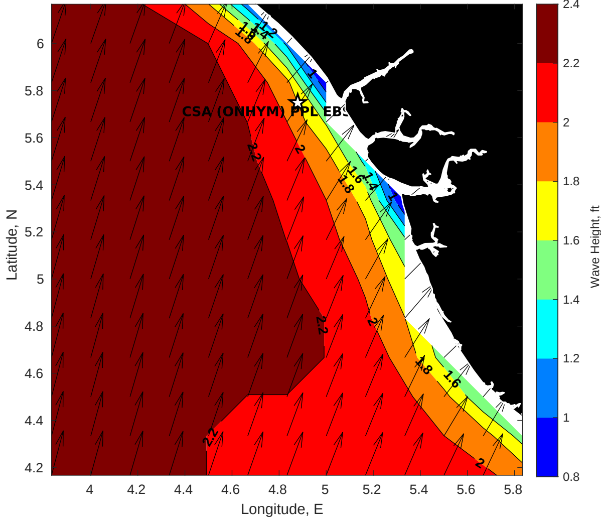
GFS Wave Height (ft) for CSA (ONHYM) PPL EBS - Nigeria at 31-Dec-2025 09:00:00
