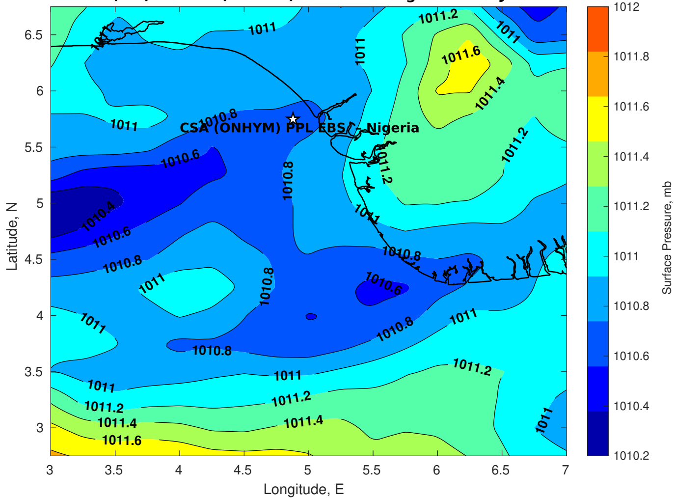
Surface Pressure (mb) for CSA (ONHYM) PPL EBS - Nigeria at 01-Jan-2026 00:00:00
