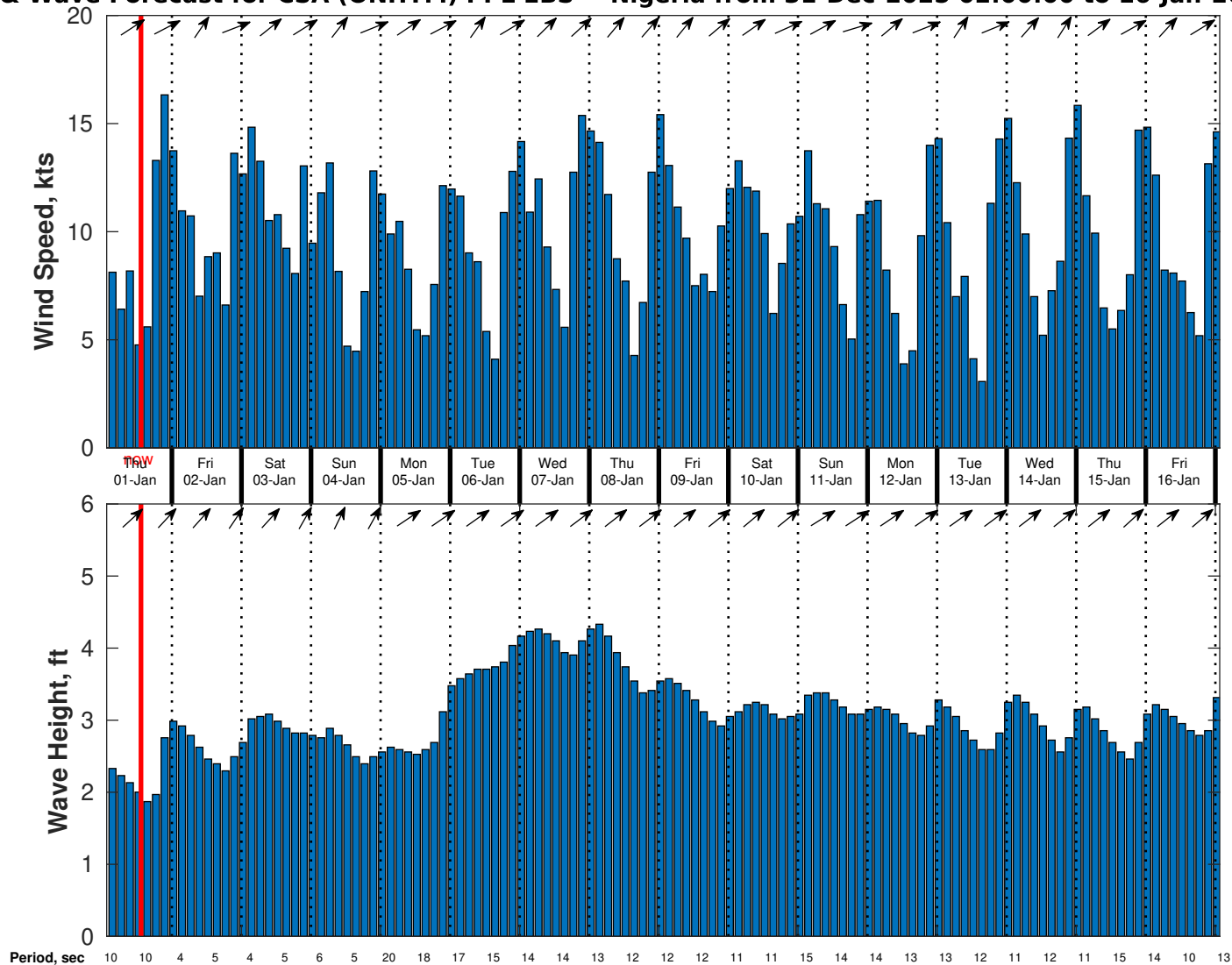
Wind & Wave Forecast for CSA (ONHYM) PPL EBS - Nigeria from 31-Dec-2025 02:00:00 to 16-Jan-2026 02:00:00
