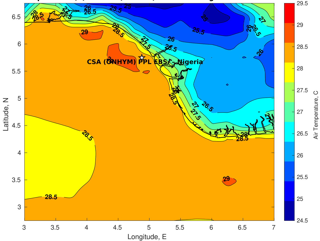
Air Temperature (C) for CSA (ONHYM) PPL EBS - Nigeria at 31-Dec-2025
