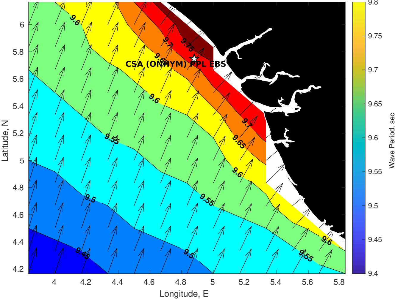
GFS Wave Period (sec) for CSA (ONHYM) PPL EBS - Nigeria at 31-Dec-2025 09:00:00
