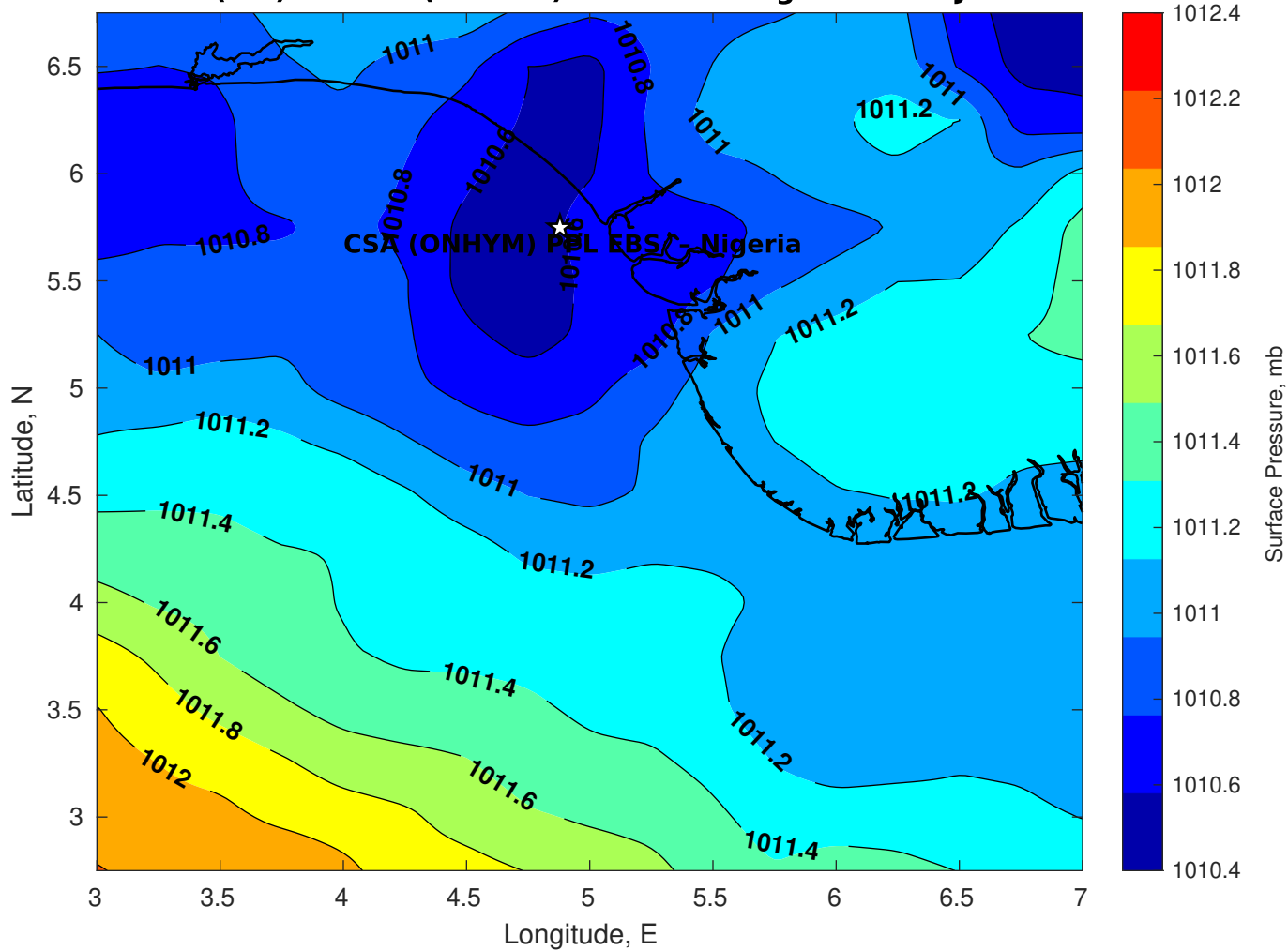
Surface Pressure (mb) for CSA (ONHYM) PPL EBS - Nigeria at 02-Jan-2026 00:00:00
