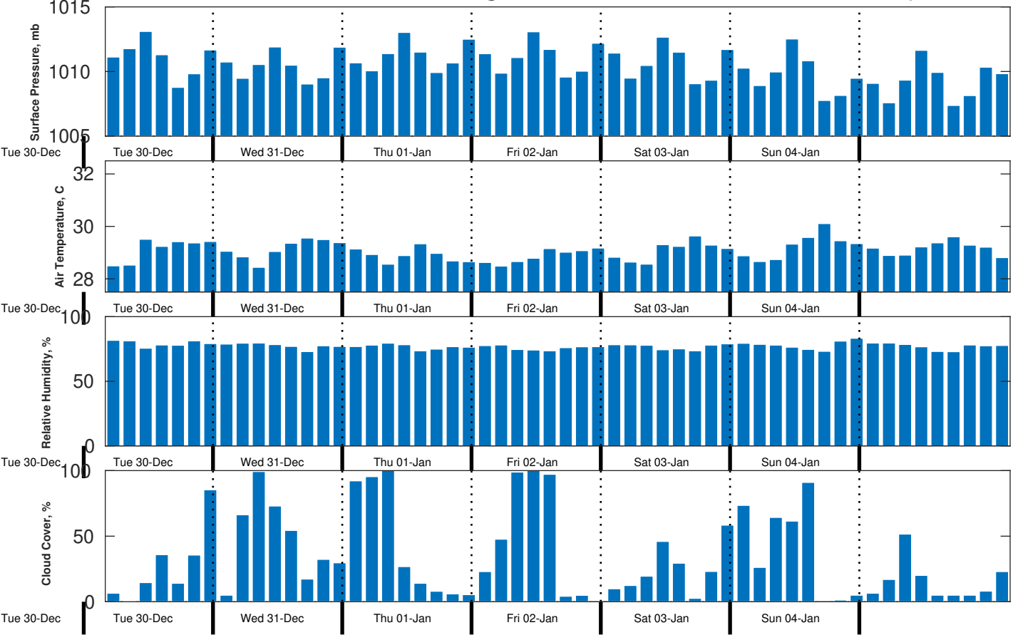
Met Forecast for CSA (ONHYM) PPL EBS - Nigeria from 31-Dec-2025 00:00:00 to 07-Jan-2026 00:00:00
