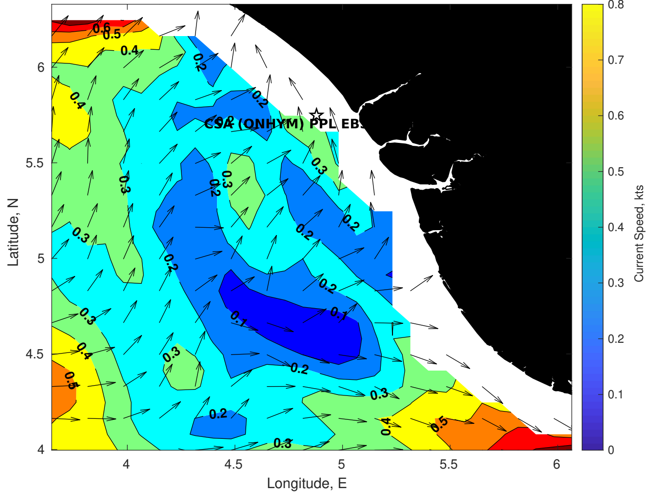
Surface Currents for CSA (ONHYM) PPL EBS - Nigeria at 30-Dec-2025 00:00:00
