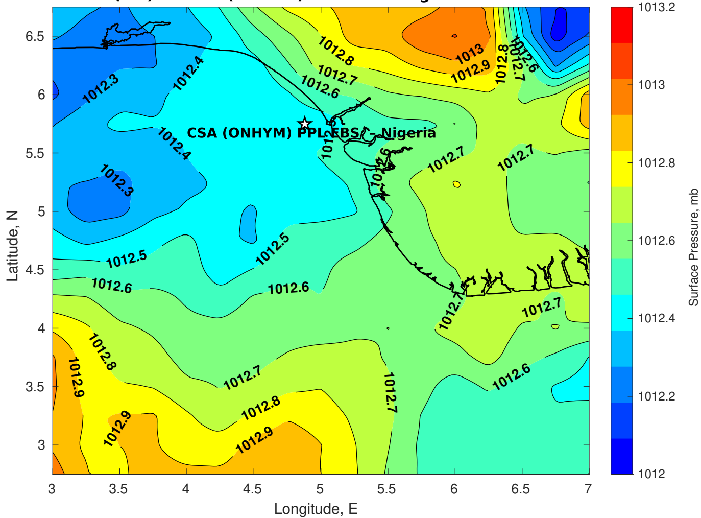
Surface Pressure (mb) for CSA (ONHYM) PPL EBS - Nigeria at 31-Dec-2025 00:00:00
