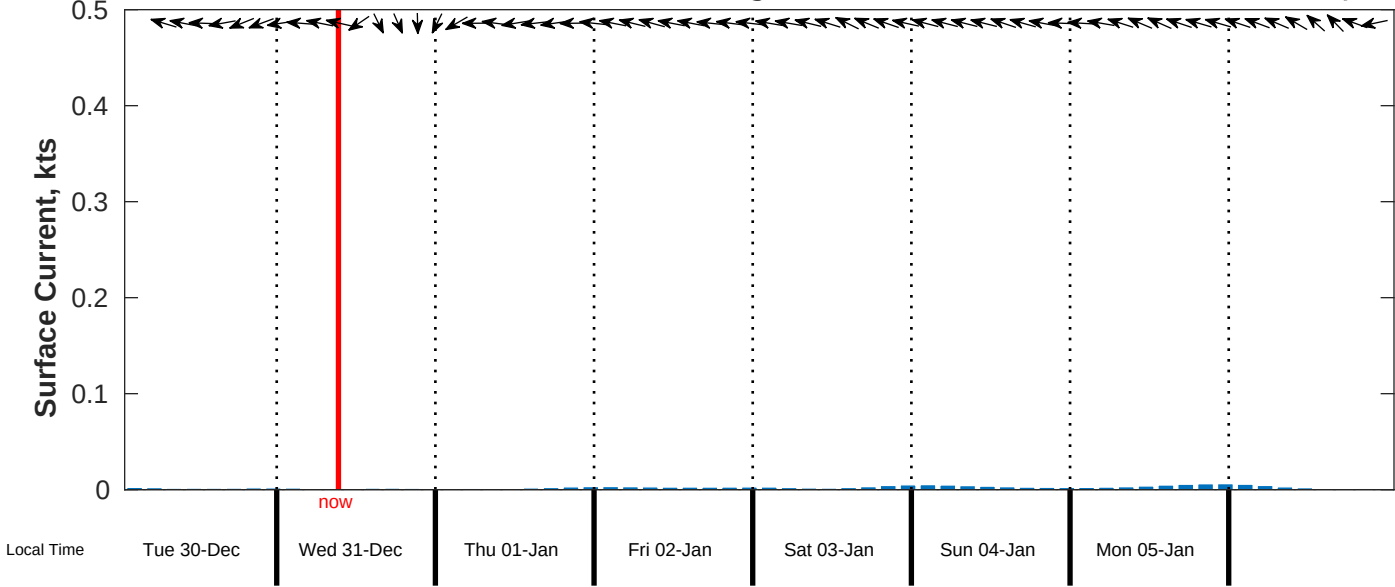
Surface Current Forecast for CSA (ONHYM) PPL EBS - Nigeria from 30-Dec-2025 00:00:00 to 07-Jan-2026 00:00:00
