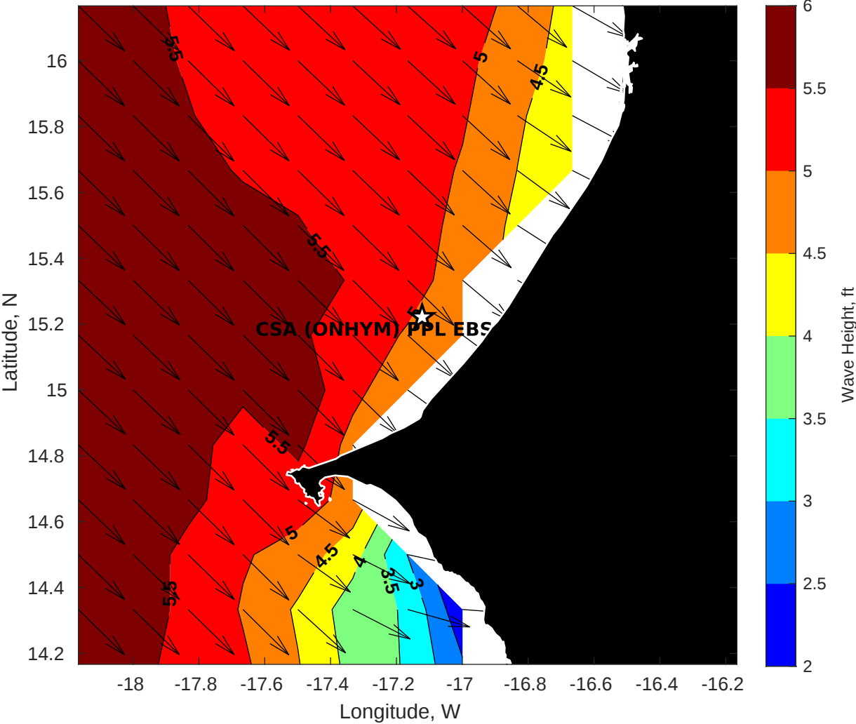
GFS Wave Height (ft) for CSA (ONHYM) PPL EBS - Senegal at 31-Dec-2025 09:00:00
