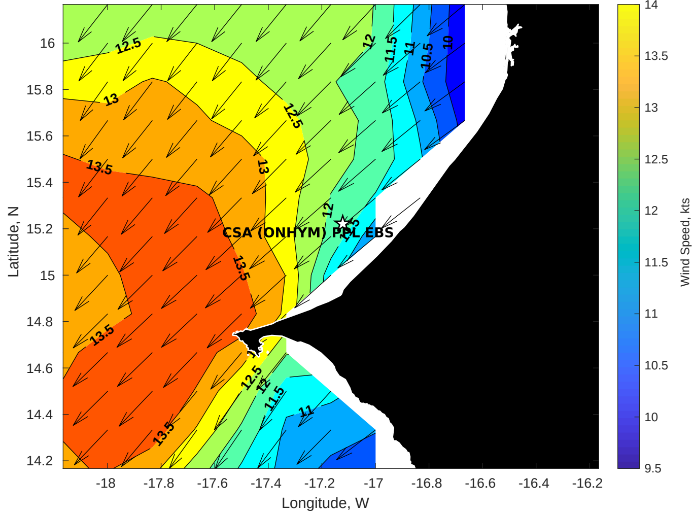
GFS Winds (kts) for CSA (ONHYM) PPL EBS - Senegal at 31-Dec-2025 09:00:00
