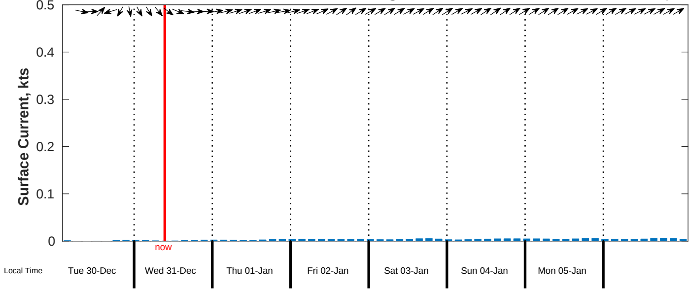
Surface Current Forecast for CSA (ONHYM) PPL EBS - Senegal from 30-Dec-2025 00:00:00 to 07-Jan-2026 00:00:00
