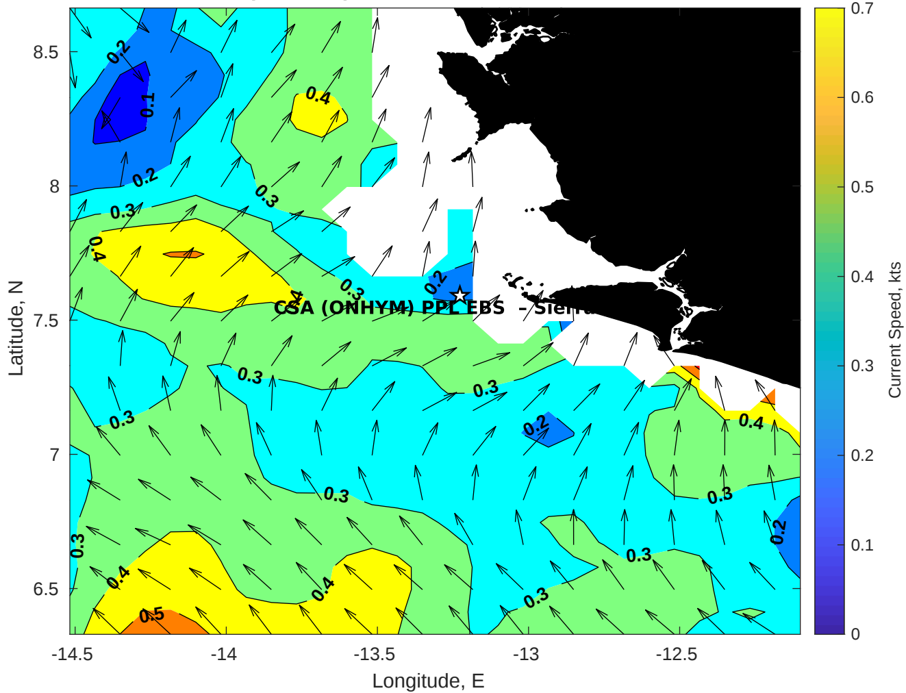
Surface Currents for CSA (ONHYM) PPL EBS - Sierra Leone at 30-Dec-2025 00:00:00
