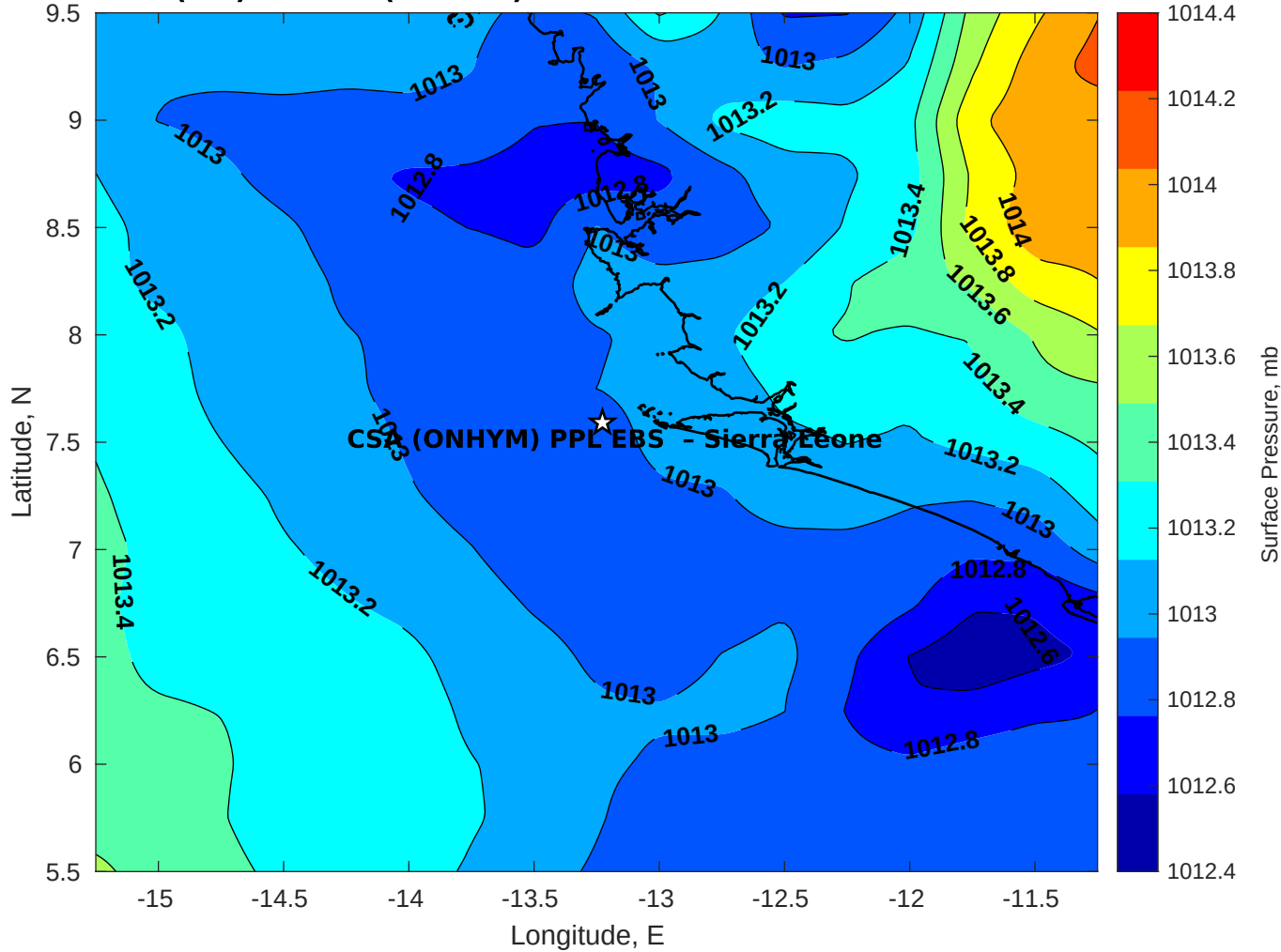
Surface Pressure (mb) for CSA (ONHYM) PPL EBS - Sierra Leone at 31-Dec-2025 00:00:00
