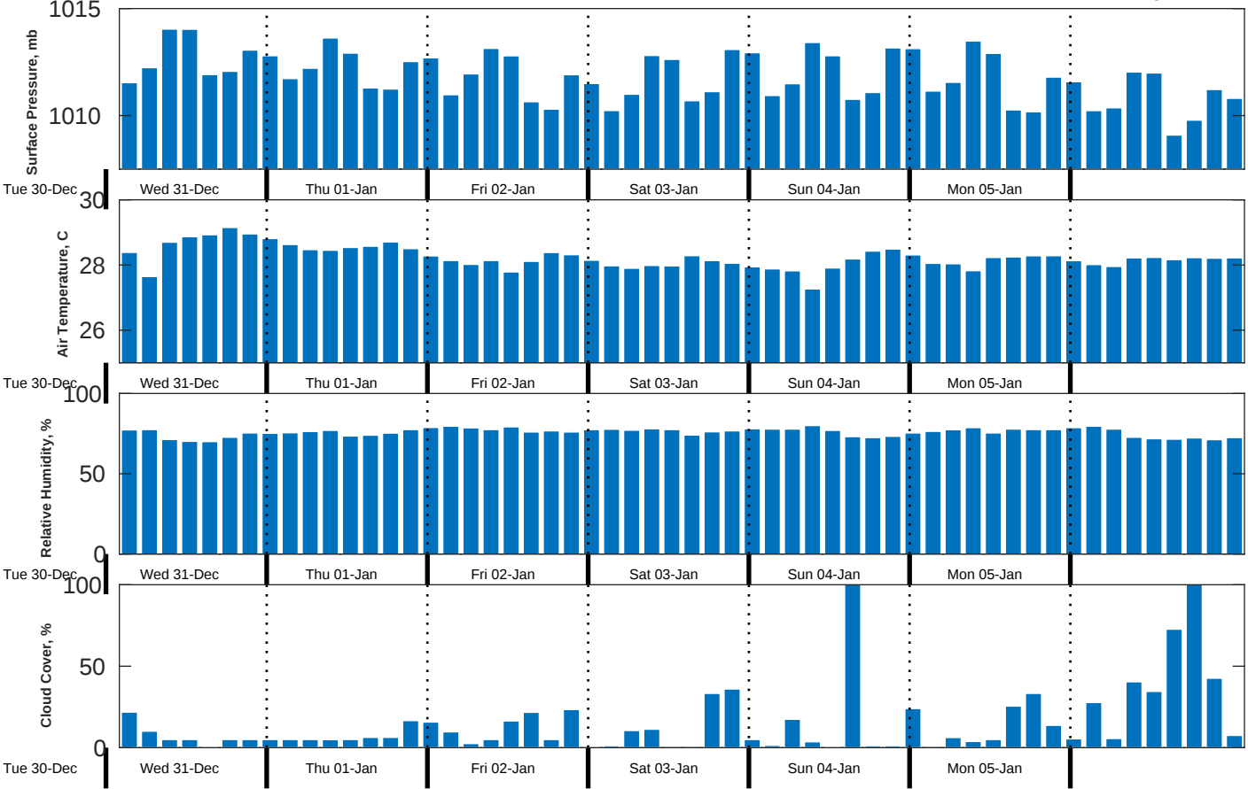
Met Forecast for CSA (ONHYM) PPL EBS - Sierra Leone from 31-Dec-2025 00:00:00 to 07-Jan-2026 00:00:00
