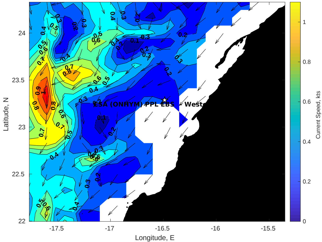
Surface Currents for CSA (ONHYM) PPL EBS - Western Sahara at 30-Dec-2025 00:00:00
