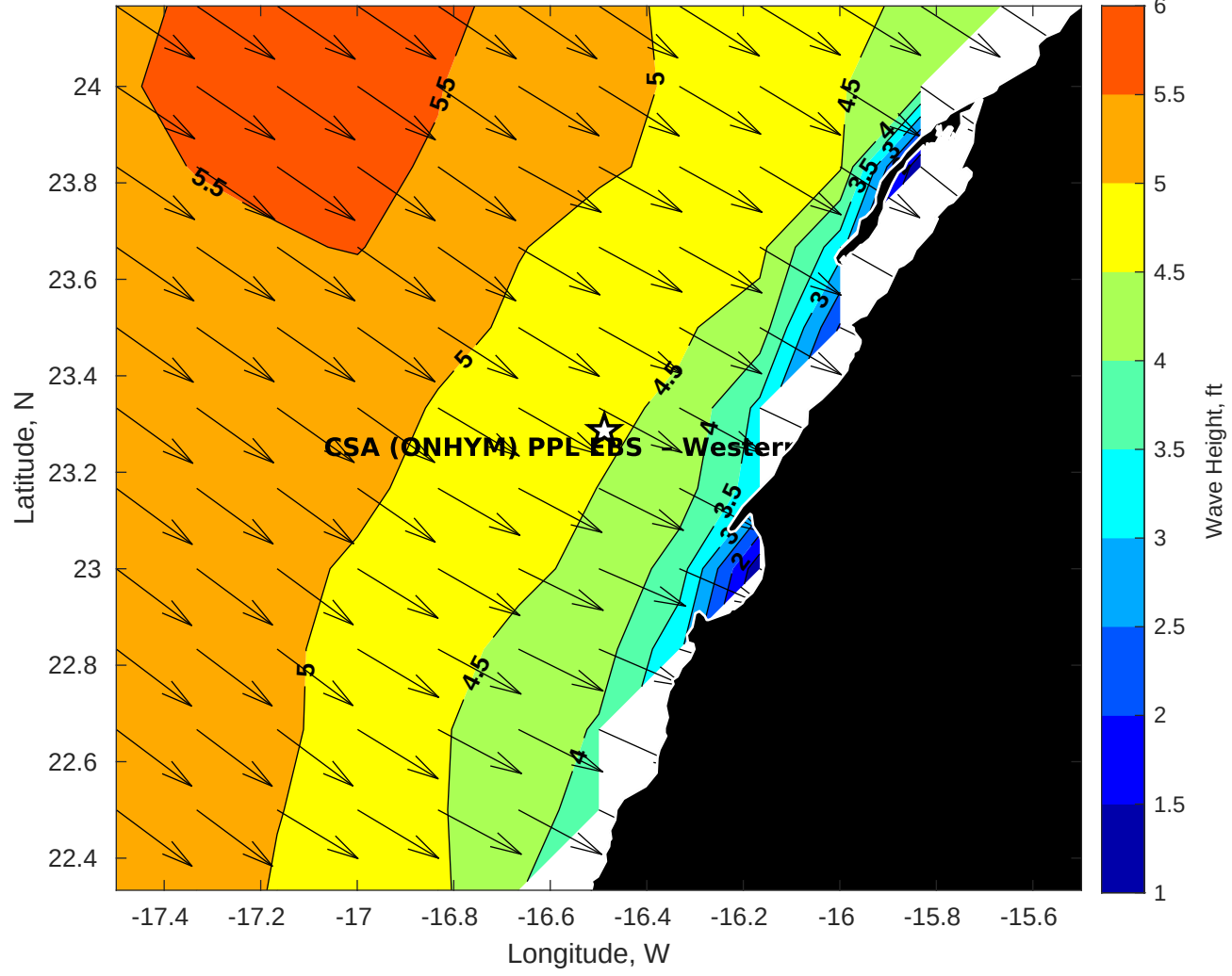
GFS Wave Height (ft) for CSA (ONHYM) PPL EBS - Western Sahara at 31-Dec-2025 09:00:00
