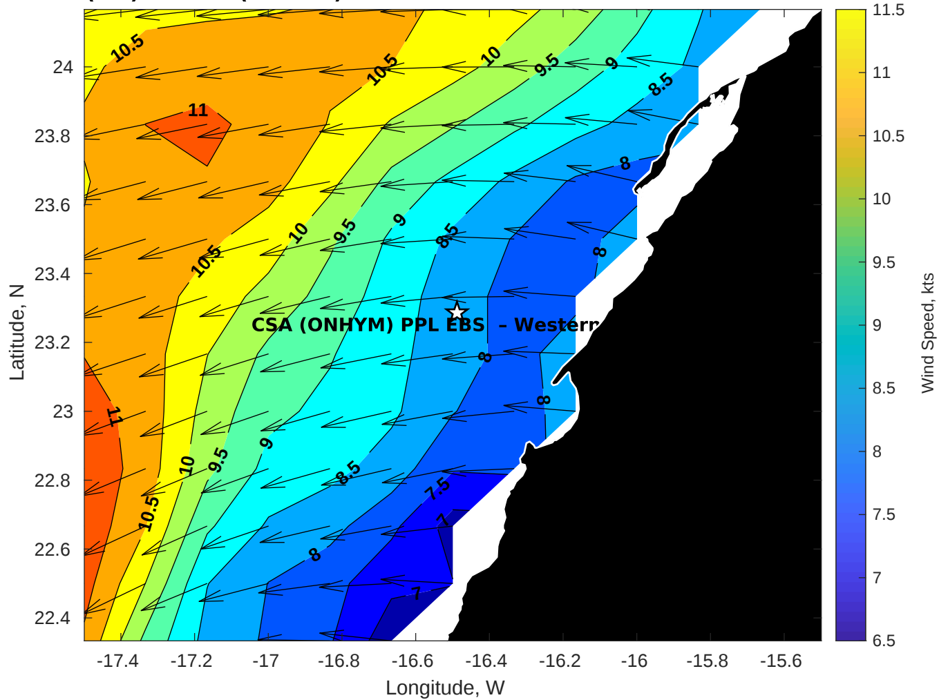
GFS Winds (kts) for CSA (ONHYM) PPL EBS - Western Sahara at 31-Dec-2025 09:00:00
