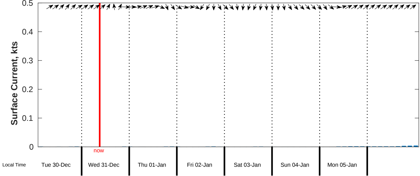
Surface Current Forecast for CSA (ONHYM) PPL EBS - Western Sahara from 30-Dec-2025 00:00:00 to 07-Jan-2026 00:00:00
