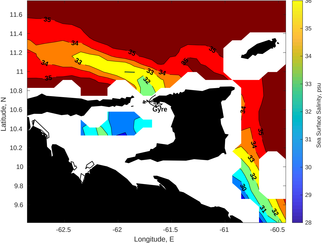
Surface Salinity for Gyre at 30-Dec-2025 00:00:00
