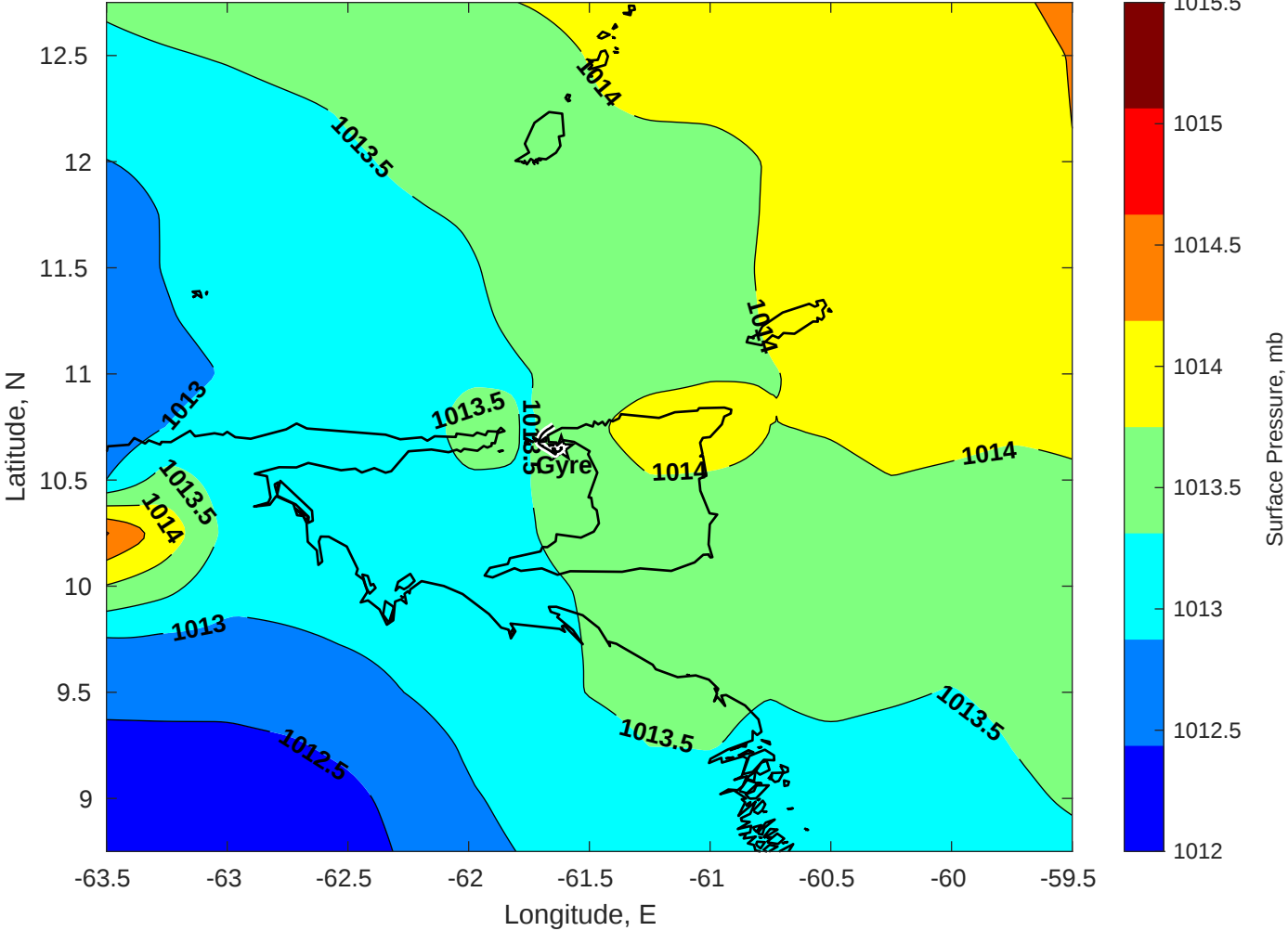
Surface Pressure (mb) for Gyre at 02-Jan-2026 00:00:00
