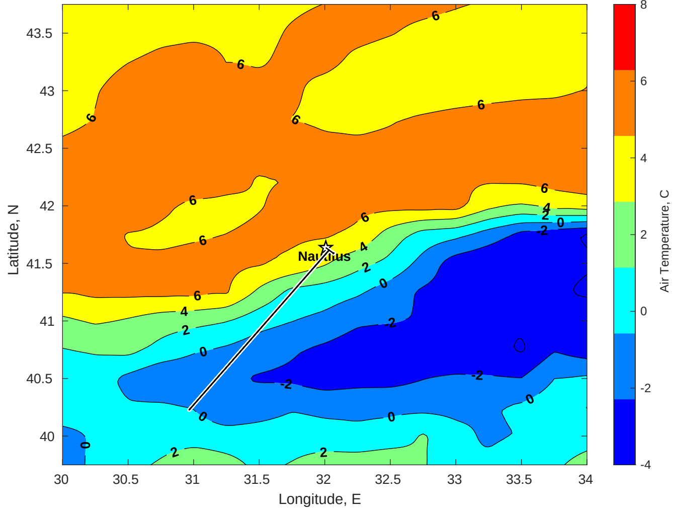
Air Temperature (C) for Nautilus at 31-Dec-2025
