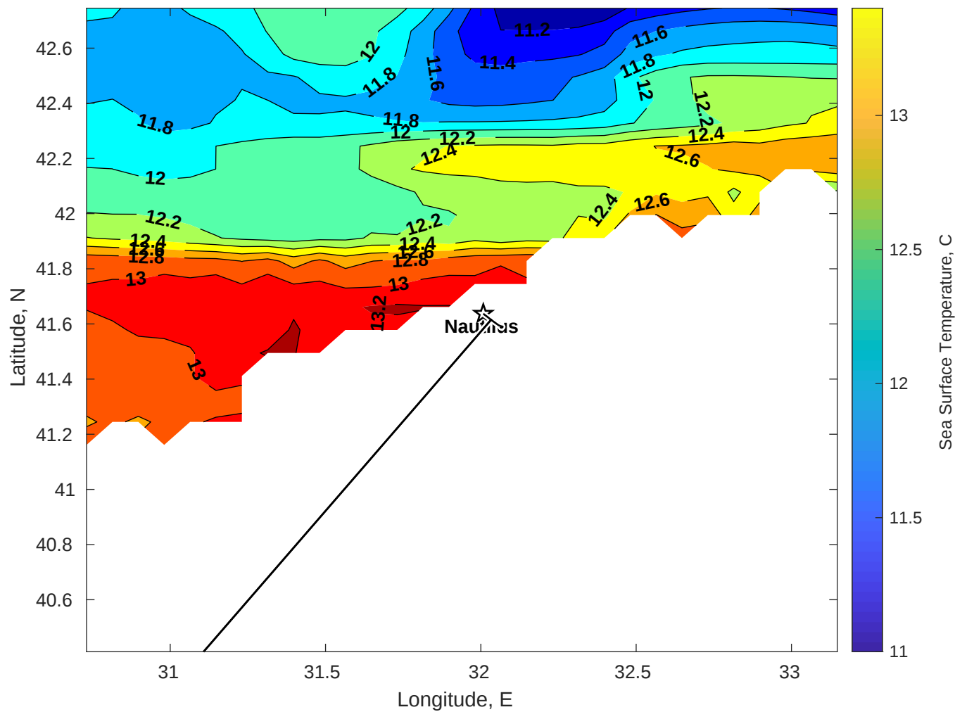
SST for Nautilus at 30-Dec-2025 00:00:00
