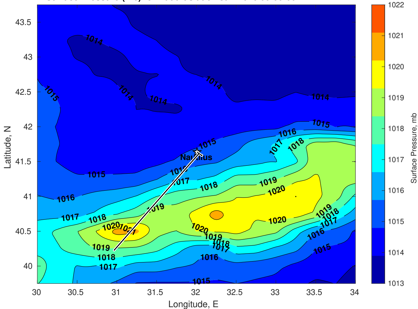
Surface Pressure (mb) for Nautilus at 01-Jan-2026 00:00:00
