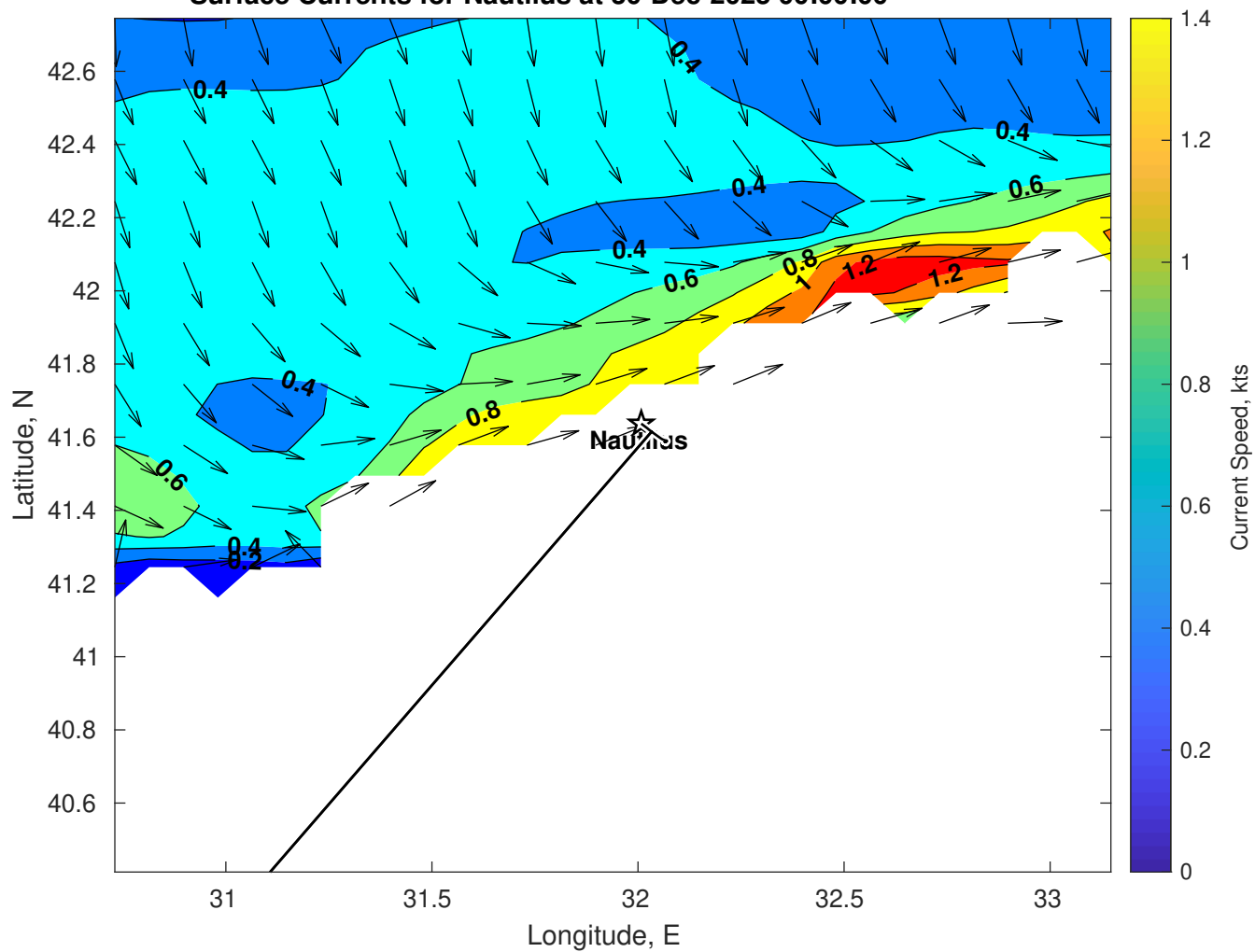
Surface Currents for Nautilus at 30-Dec-2025 00:00:00
