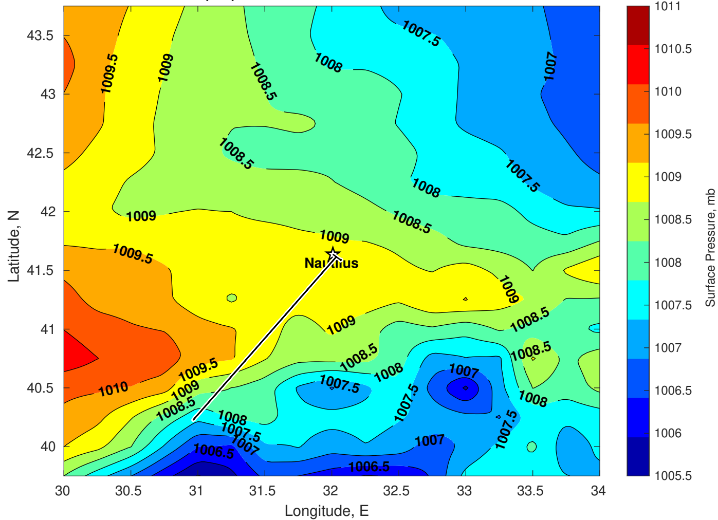
Surface Pressure (mb) for Nautilus at 31-Dec-2025 00:00:00
