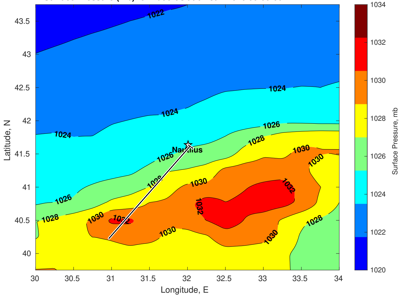
Surface Pressure (mb) for Nautilus at 02-Jan-2026 00:00:00
