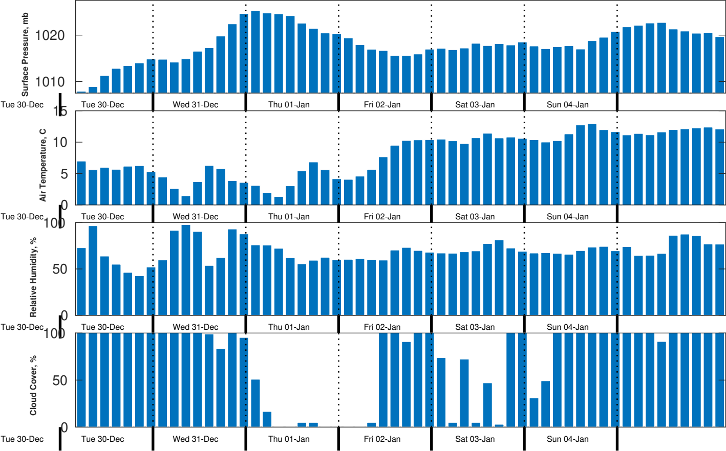
Met Forecast for Nautilus from 31-Dec-2025 00:00:00 to 07-Jan-2026 00:00:00
