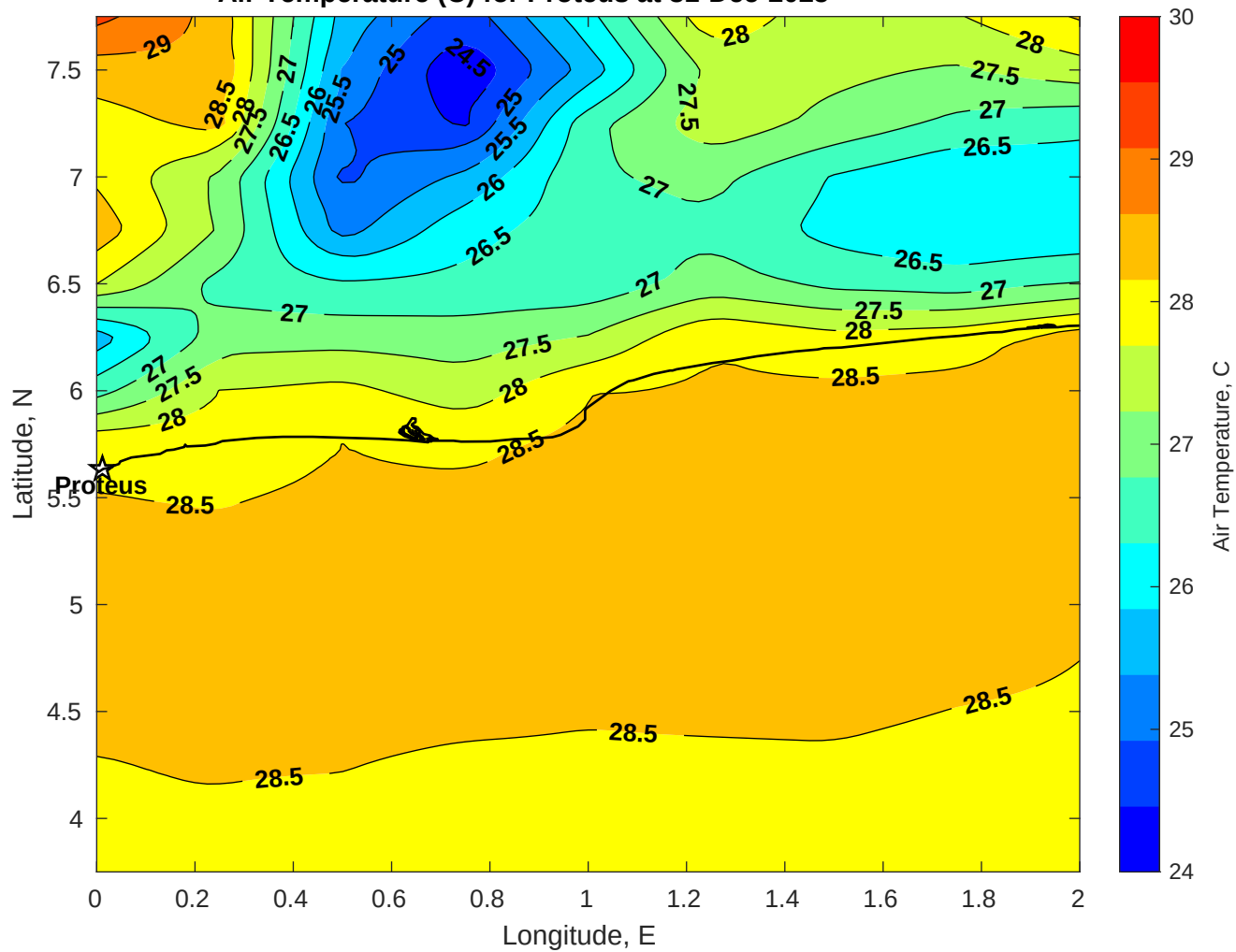
Air Temperature (C) for Proteus at 31-Dec-2025
