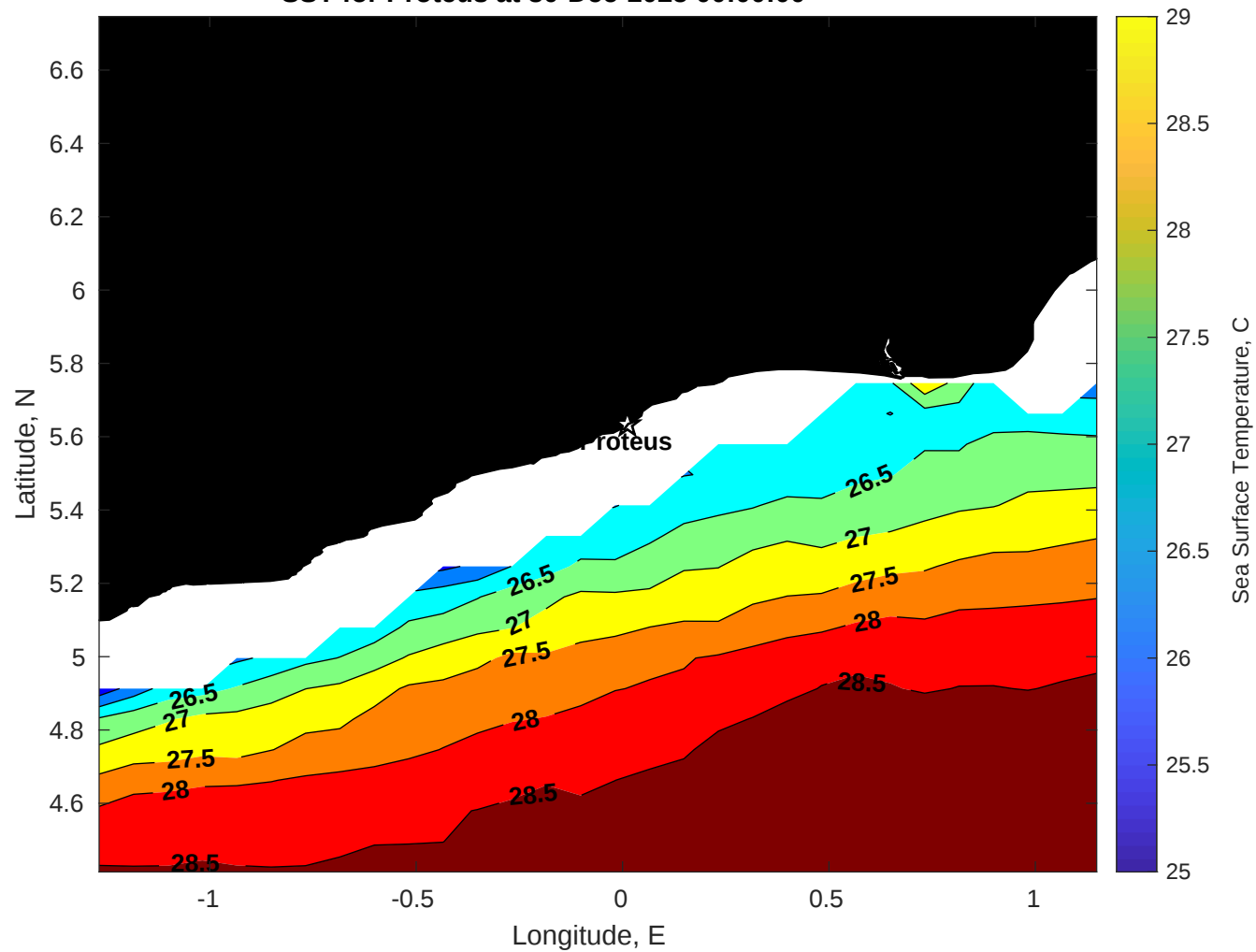
SST for Proteus at 30-Dec-2025 00:00:00
