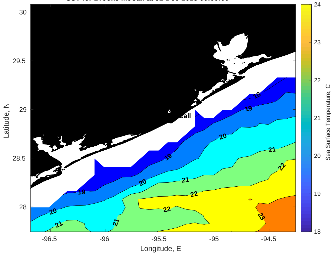
SST for Brooks McCall at 31-Dec-2025 00:00:00
