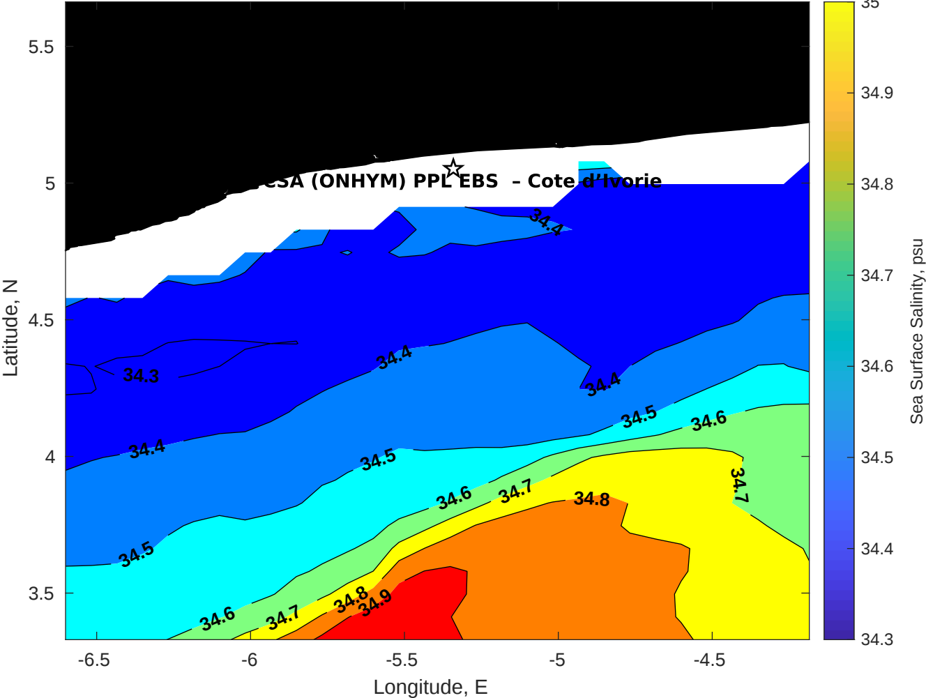
Surface Salinity for CSA (ONHYM) PPL EBS - Cote d'Ivoire at 31-Dec-2025 00:00:00
