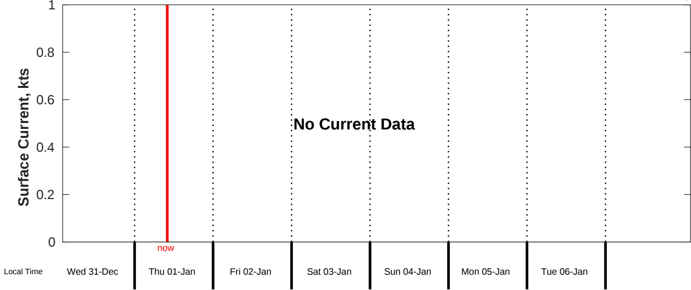
Surface Current Forecast for CSA (ONHYM) PPL EBS - Cote d'Ivoire from 31-Dec-2025 00:00:00 to 08-Jan-2026 00:00:00
