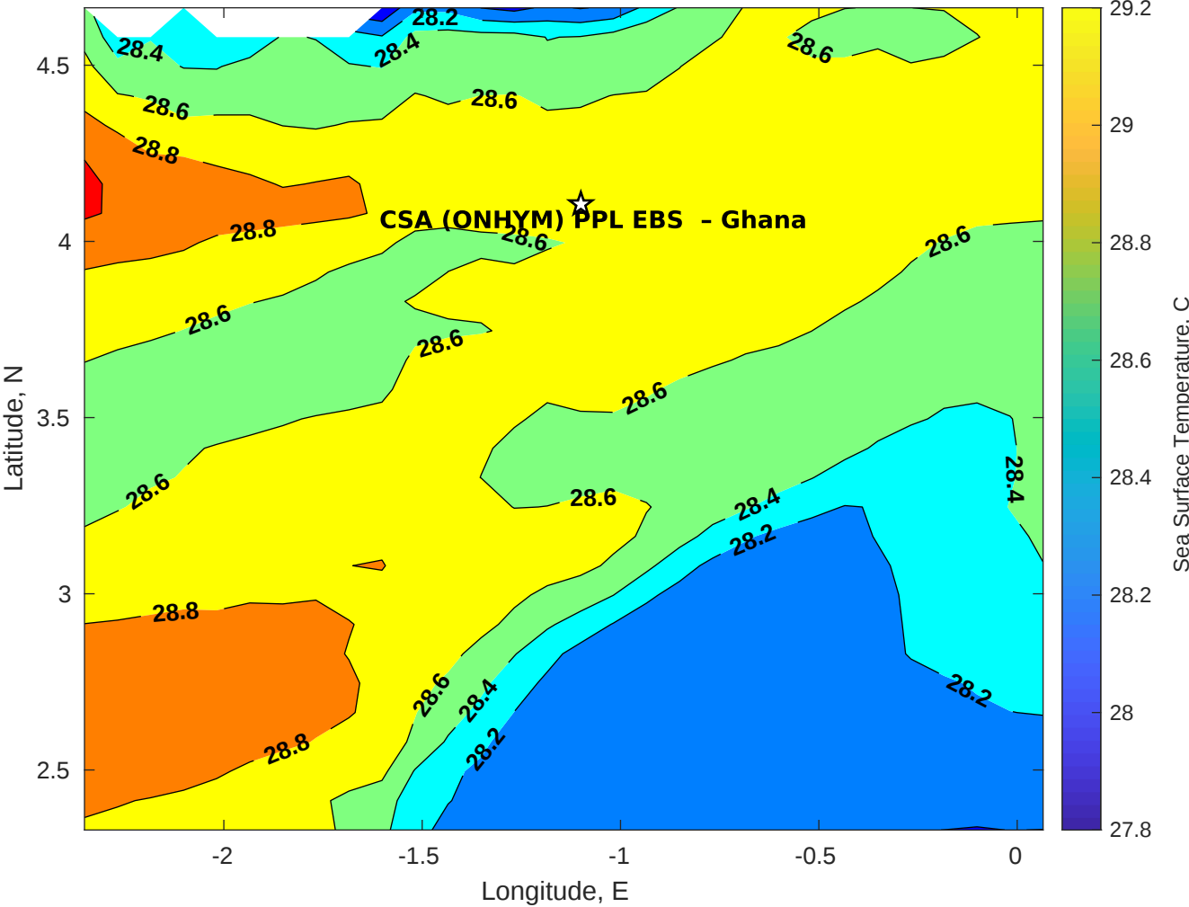
SST for CSA (ONHYM) PPL EBS - Ghana at 31-Dec-2025 00:00:00
