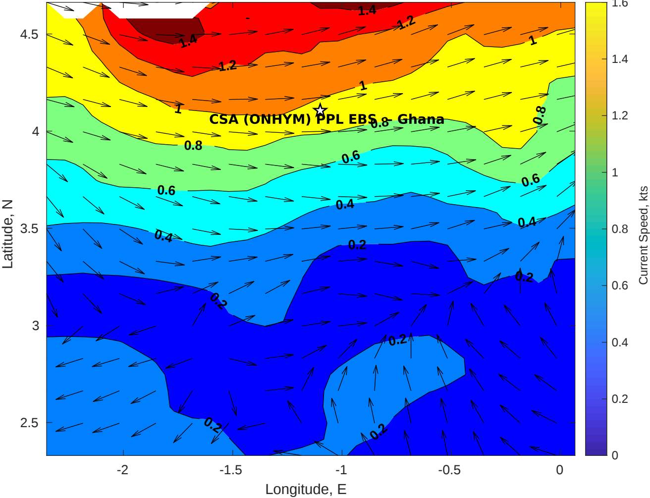
Surface Currents for CSA (ONHYM) PPL EBS - Ghana at 31-Dec-2025 00:00:00
