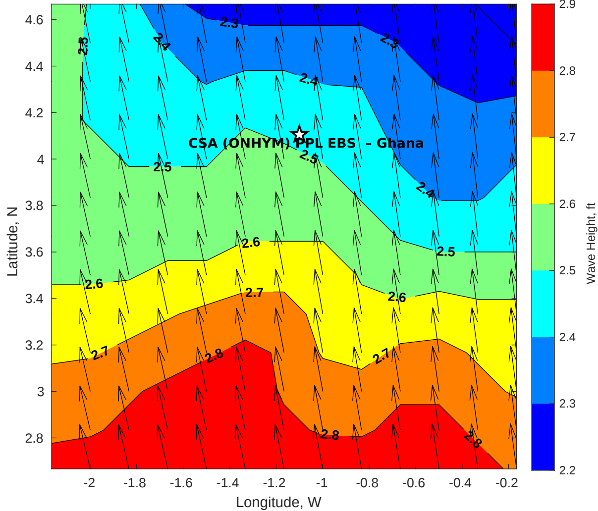
GFS Wave Height (ft) for CSA (ONHYM) PPL EBS - Ghana at 01-Jan-2026 09:00:00
