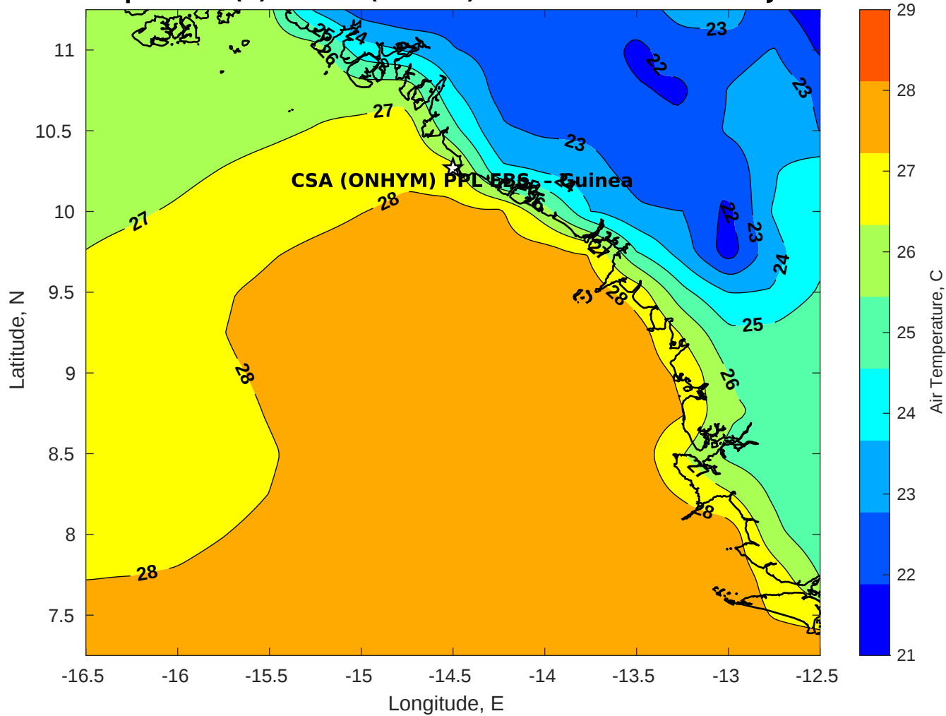
Air Temperature (C) for CSA (ONHYM) PPL EBS - Guinea at 01-Jan-2026
