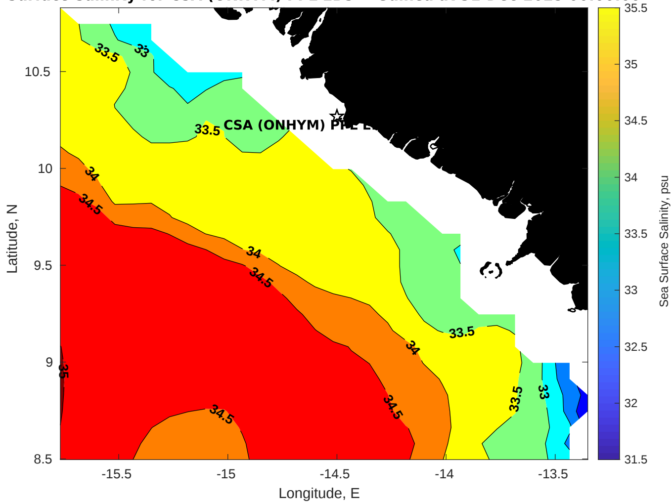
Surface Salinity for CSA (ONHYM) PPL EBS - Guinea at 31-Dec-2025 00:00:00
