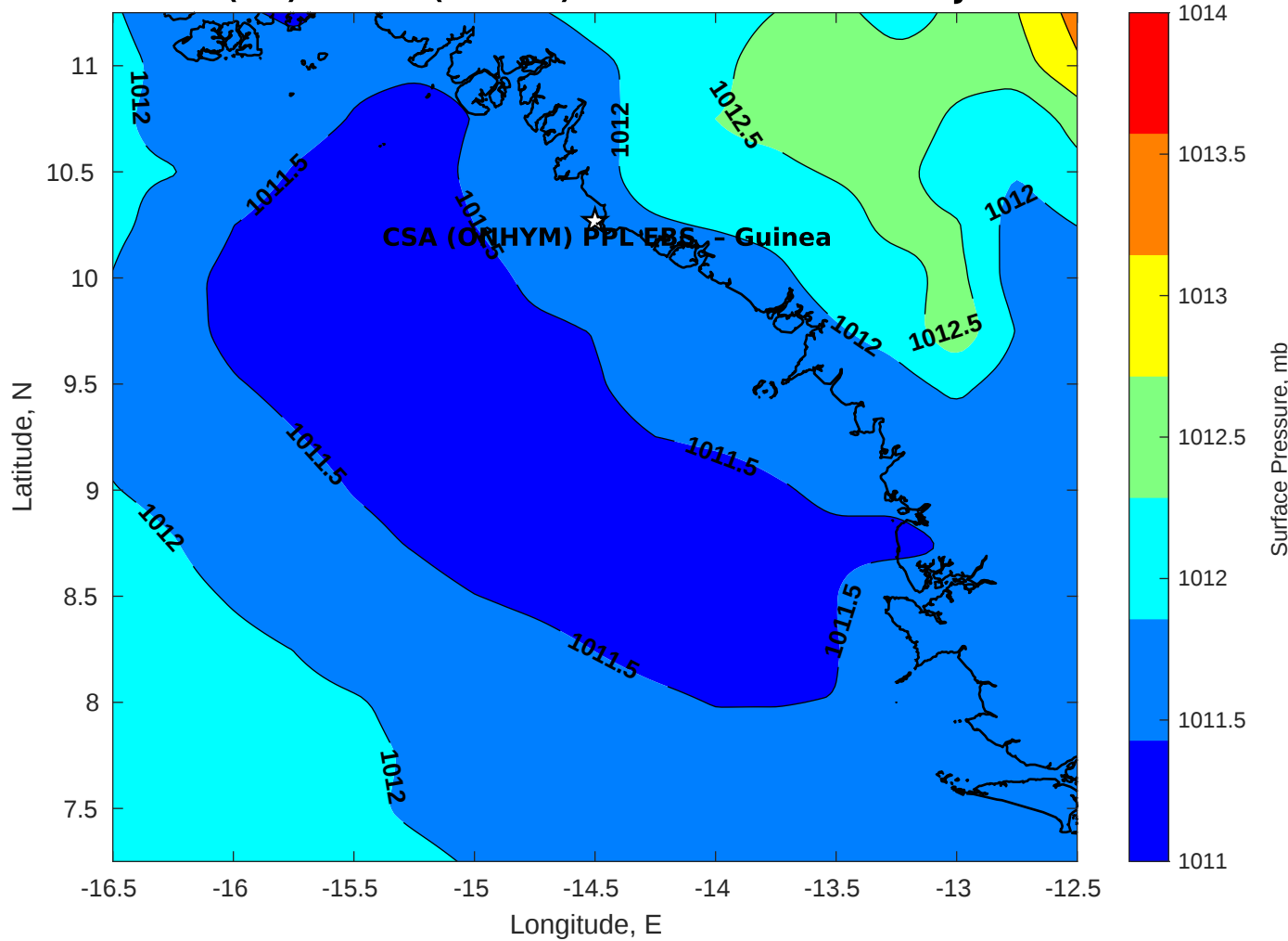
Surface Pressure (mb) for CSA (ONHYM) PPL EBS - Guinea at 03-Jan-2026 00:00:00
