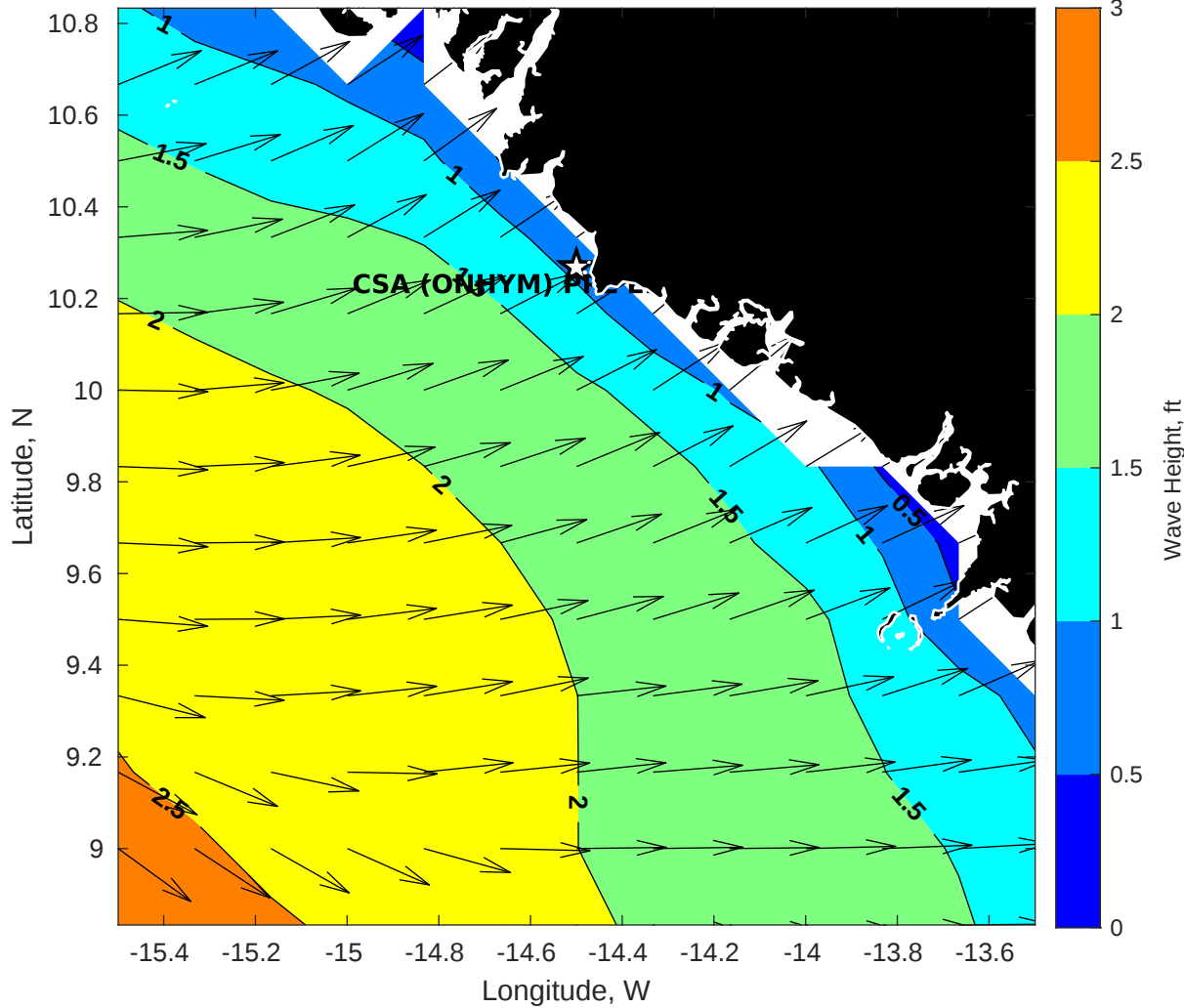
GFS Wave Height (ft) for CSA (ONHYM) PPL EBS - Guinea at 01-Jan-2026 09:00:00
