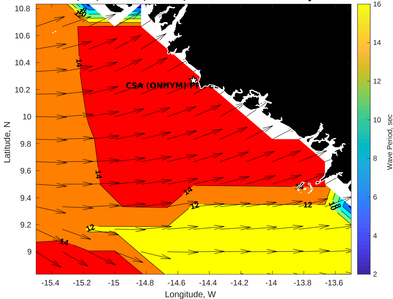
GFS Wave Period (sec) for CSA (ONHYM) PPL EBS - Guinea at 01-Jan-2026 09:00:00
