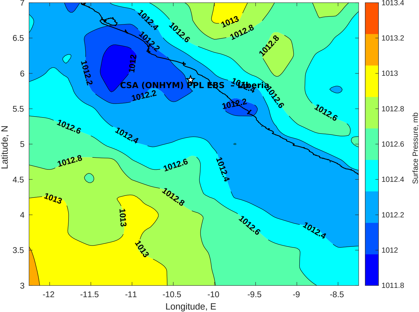
Surface Pressure (mb) for CSA (ONHYM) PPL EBS - Liberia at 01-Jan-2026 00:00:00
