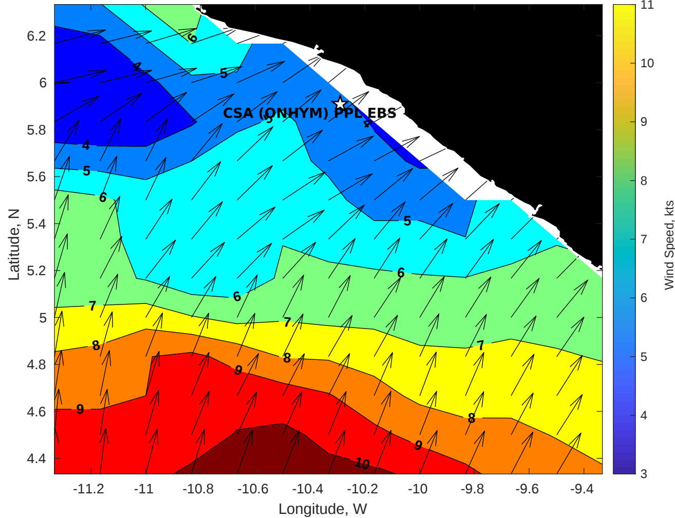
GFS Winds (kts) for CSA (ONHYM) PPL EBS - Liberia at 01-Jan-2026 09:00:00
