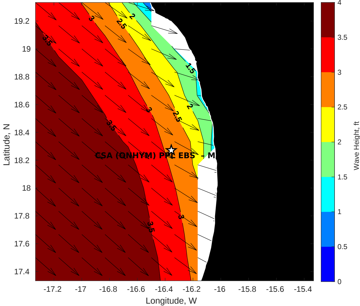
GFS Wave Height (ft) for CSA (ONHYM) PPL EBS - Mauritania at 01-Jan-2026 09:00:00
