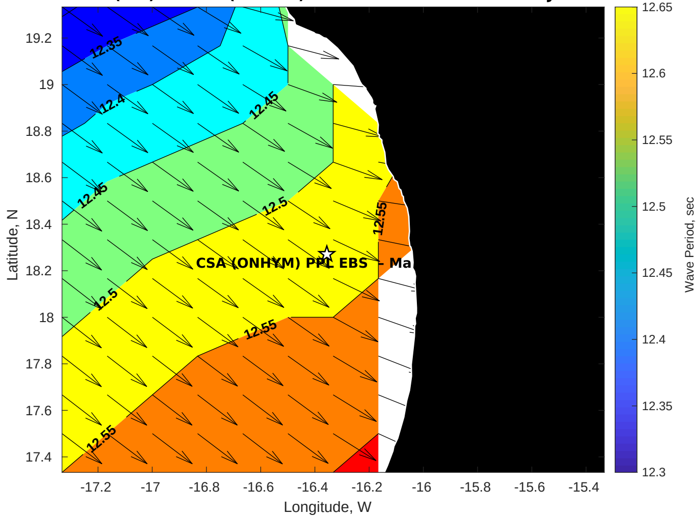
GFS Wave Period (sec) for CSA (ONHYM) PPL EBS - Mauritania at 01-Jan-2026 09:00:00
