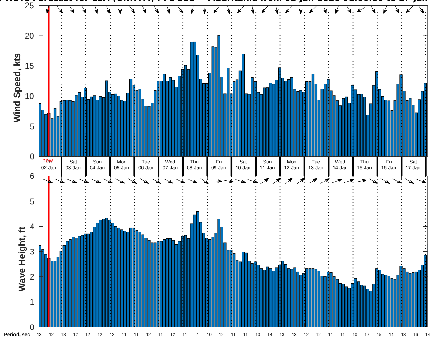
Wind & Wave Forecast for CSA (ONHYM) PPL EBS - Mauritania from 01-Jan-2026 01:00:00 to 17-Jan-2026 01:00:00
