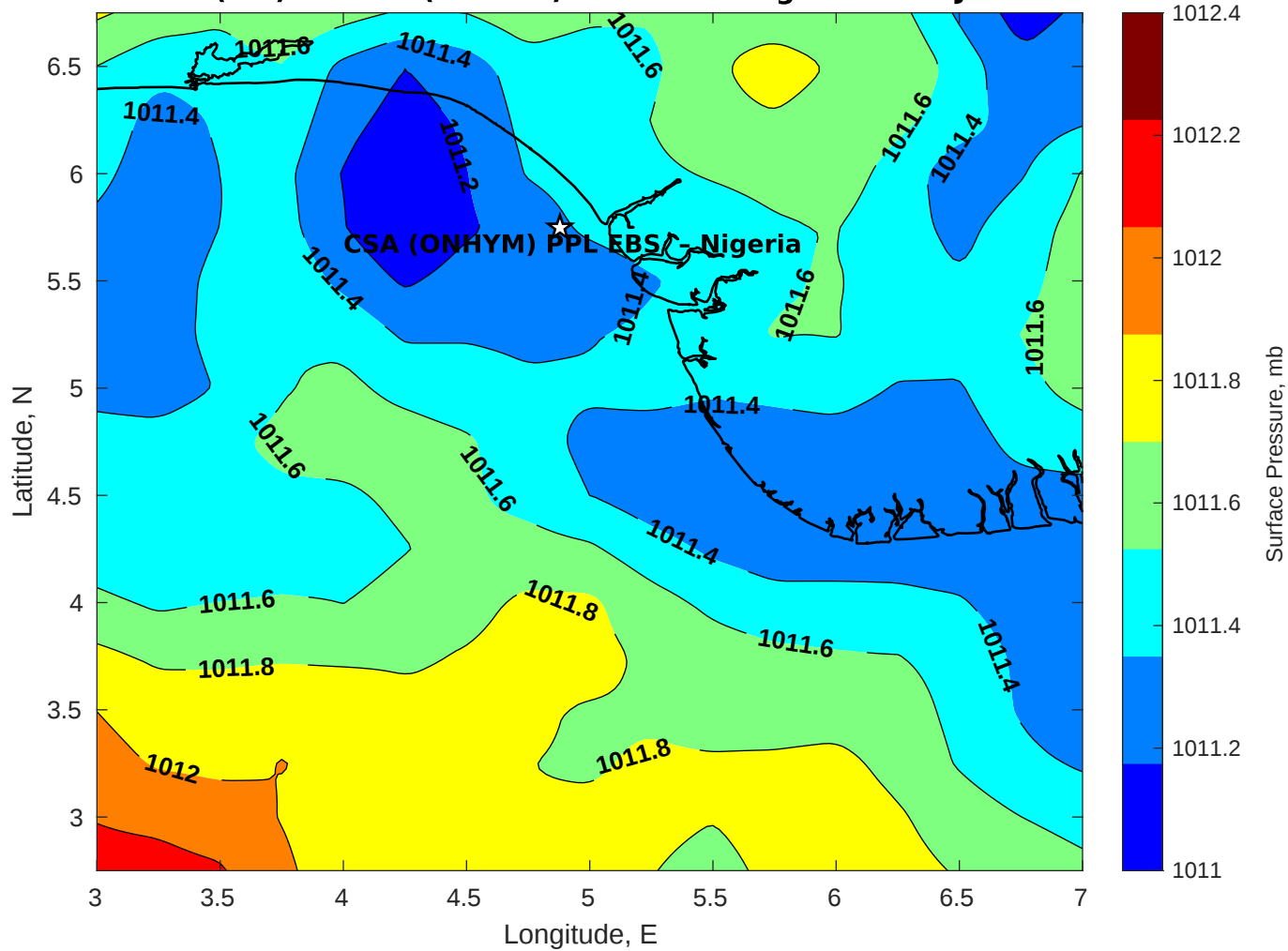
Surface Pressure (mb) for CSA (ONHYM) PPL EBS - Nigeria at 03-Jan-2026 00:00:00
