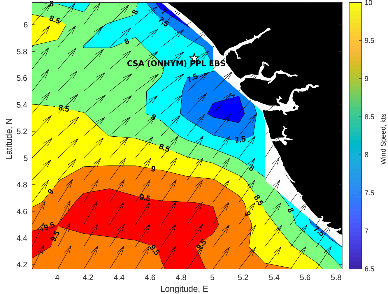
GFS Winds (kts) for CSA (ONHYM) PPL EBS - Nigeria at 01-Jan-2026 09:00:00
